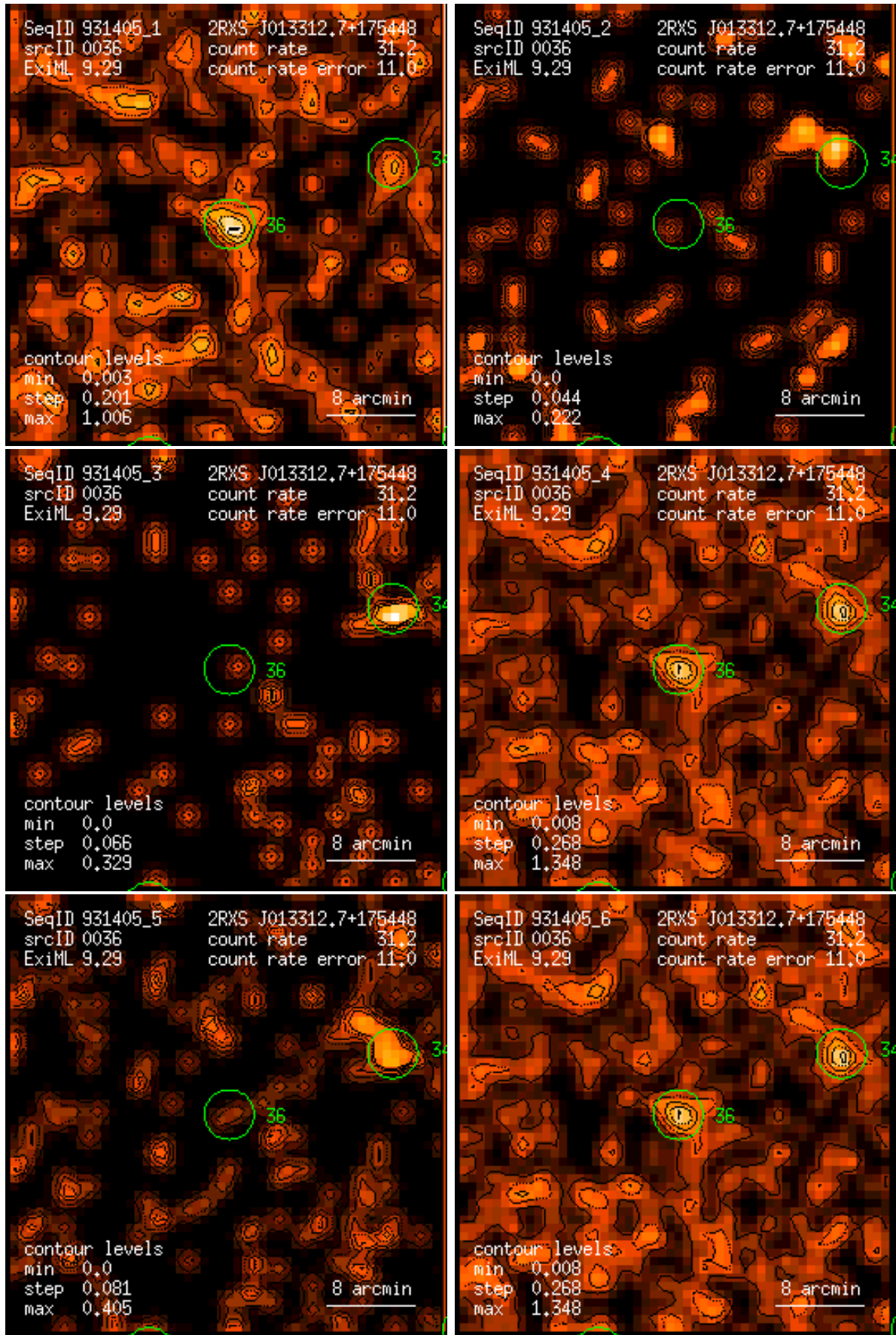
Figure 36: RASS 931405: detection 0036: band rate images, Gaussian filter: (1) PSPC channels 11 – 41, (2) 52 – 90, (3) 91 – 201, (4) 11 – 235, (5) 52 – 201, (6) 11 – 201. Broad band rates in counts/ks. Band rate contour levels in counts/ks/arcmin 2 .
