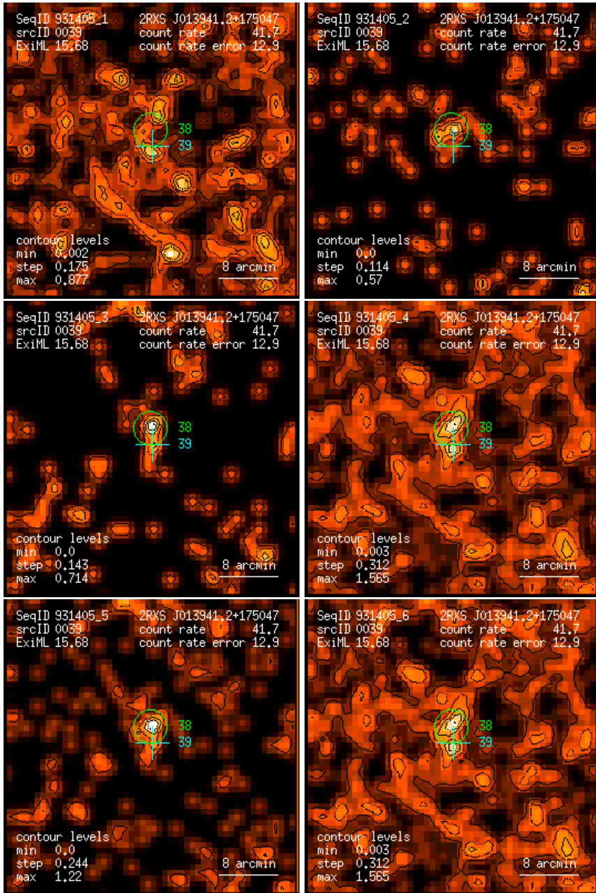
Figure 39: RASS 931405: detection 0039: band rate images, Gaussian filter: (1) PSPC channels 11 – 41, (2) 52 – 90, (3) 91 – 201, (4) 11 – 235, (5) 52 – 201, (6) 11 – 201. Broad band rates in counts/ks. Band rate contour levels in counts/ks/arcmin 2 .
