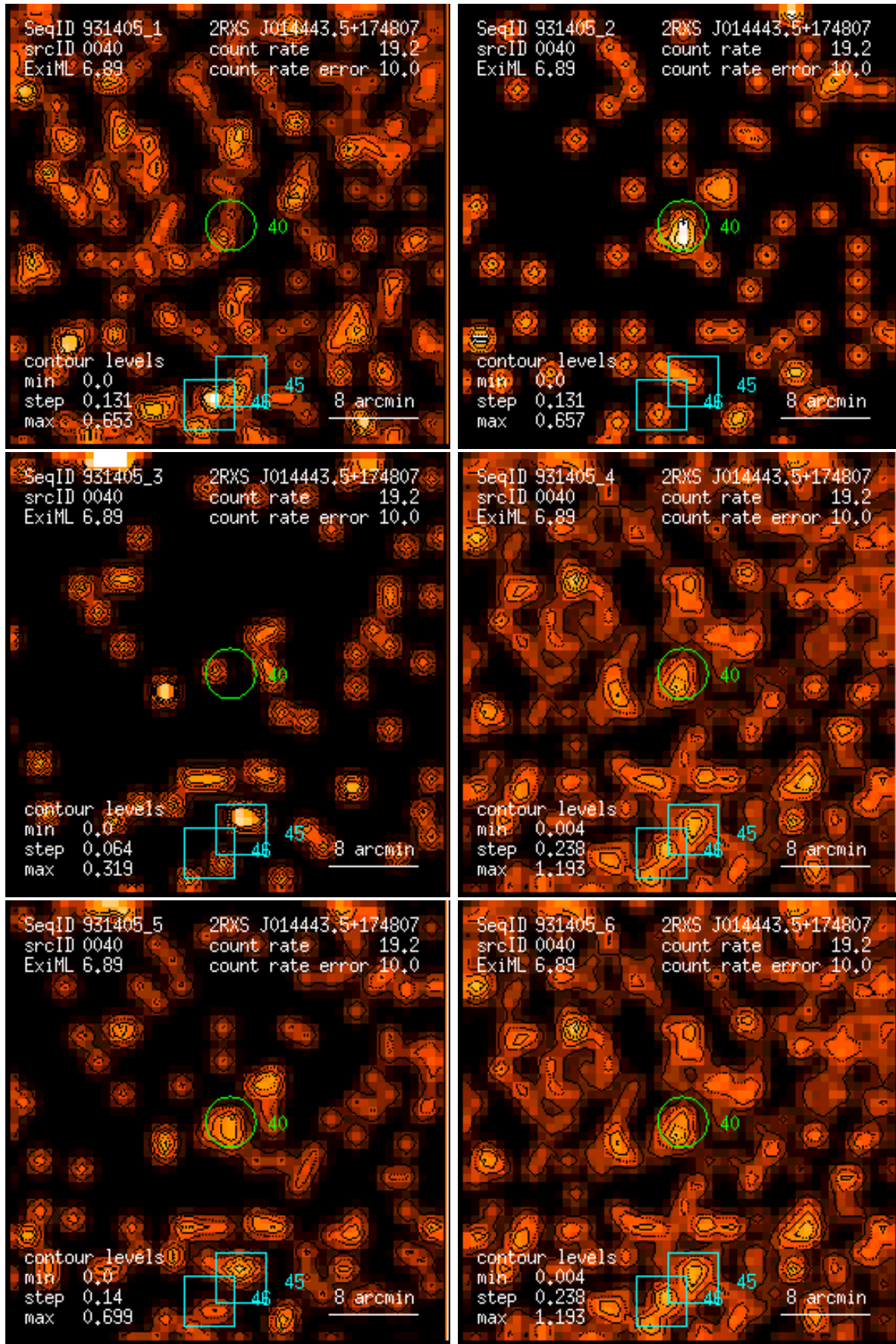
Figure 40: RASS 931405: detection 0040: band rate images, Gaussian filter: (1) PSPC channels 11 – 41, (2) 52 – 90, (3) 91 – 201, (4) 11 – 235, (5) 52 – 201, (6) 11 – 201. Broad band rates in counts/ks. Band rate contour levels in counts/ks/arcmin 2 .
