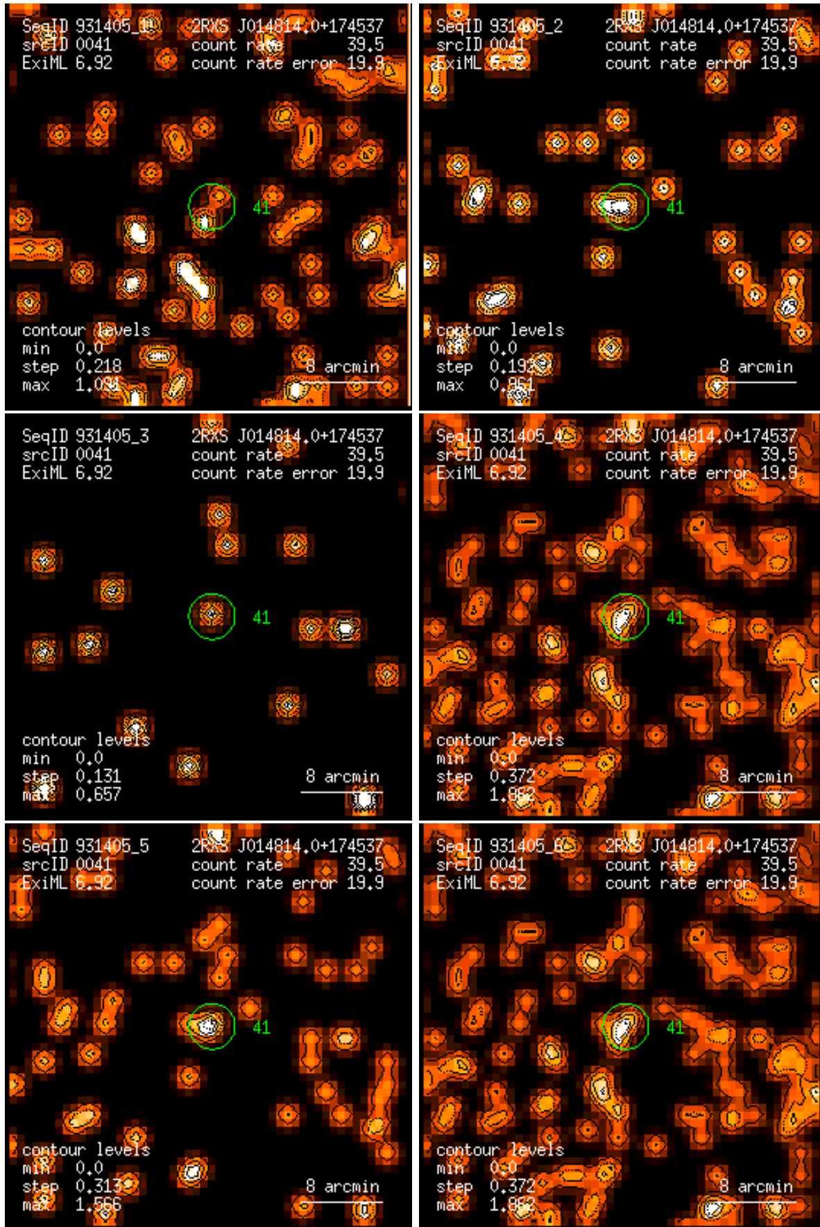
Figure 41: RASS 931405: detection 0041: band rate images, Gaussian filter: (1) PSPC channels 11 – 41, (2) 52 – 90, (3) 91 – 201, (4) 11 – 235, (5) 52 – 201, (6) 11 – 201. Broad band rates in counts/ks. Band rate contour levels in counts/ks/arcmin 2 .
