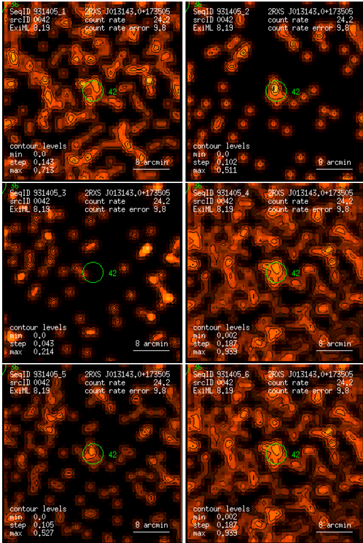
Figure 42: RASS 931405: detection 0042: band rate images, Gaussian filter: (1) PSPC channels 11 – 41, (2) 52 – 90, (3) 91 – 201, (4) 11 – 235, (5) 52 – 201, (6) 11 – 201. Broad band rates in counts/ks. Band rate contour levels in counts/ks/arcmin 2 .
