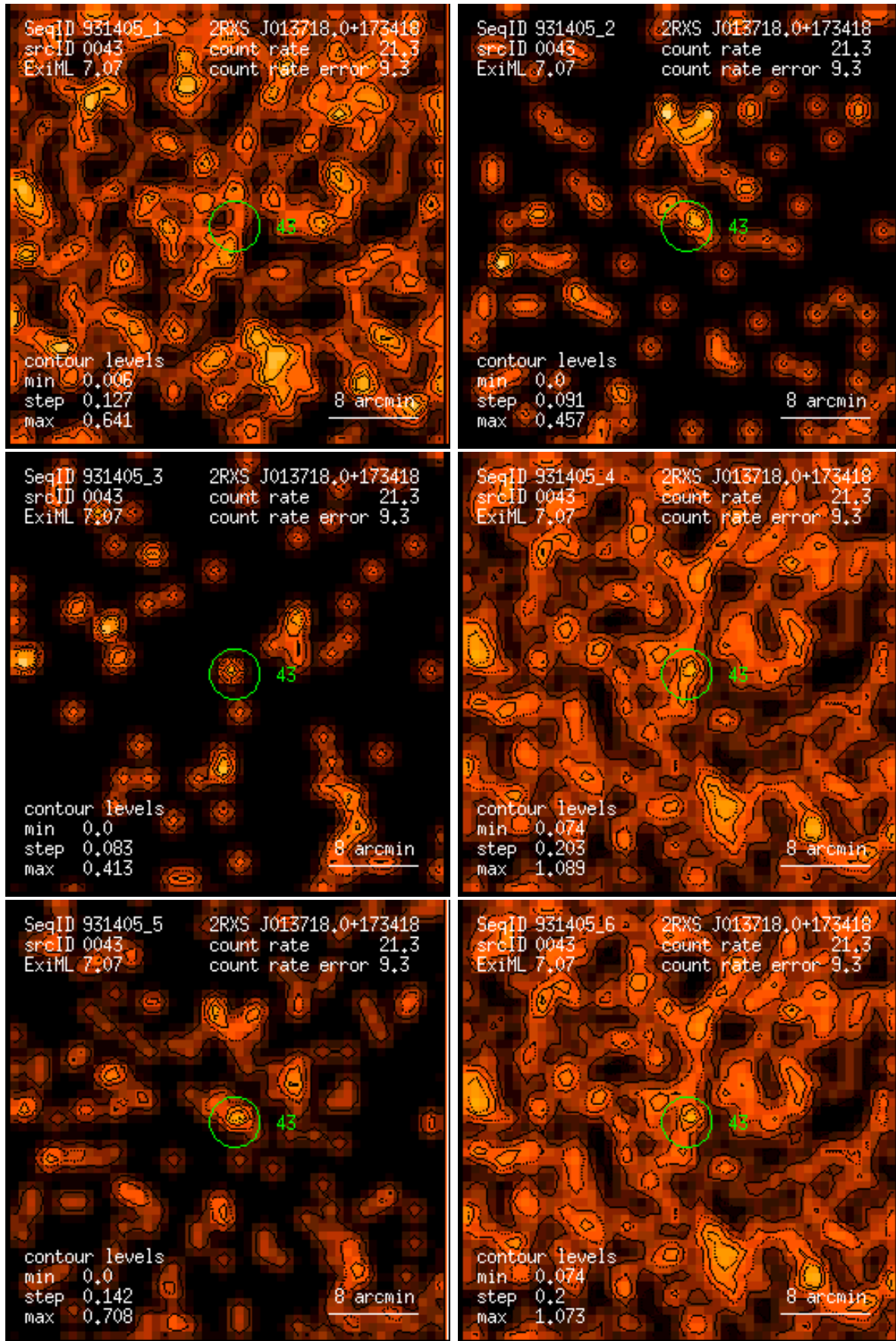
Figure 43: RASS 931405: detection 0043: band rate images, Gaussian filter: (1) PSPC channels 11 – 41, (2) 52 – 90, (3) 91 – 201, (4) 11 – 235, (5) 52 – 201, (6) 11 – 201. Broad band rates in counts/ks. Band rate contour levels in counts/ks/arcmin 2 .
