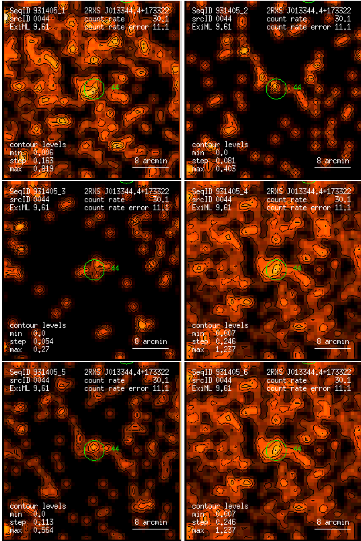
Figure 44: RASS 931405: detection 0044: band rate images, Gaussian filter: (1) PSPC channels 11 – 41, (2) 52 – 90, (3) 91 – 201, (4) 11 – 235, (5) 52 – 201, (6) 11 – 201. Broad band rates in counts/ks. Band rate contour levels in counts/ks/arcmin 2 .
