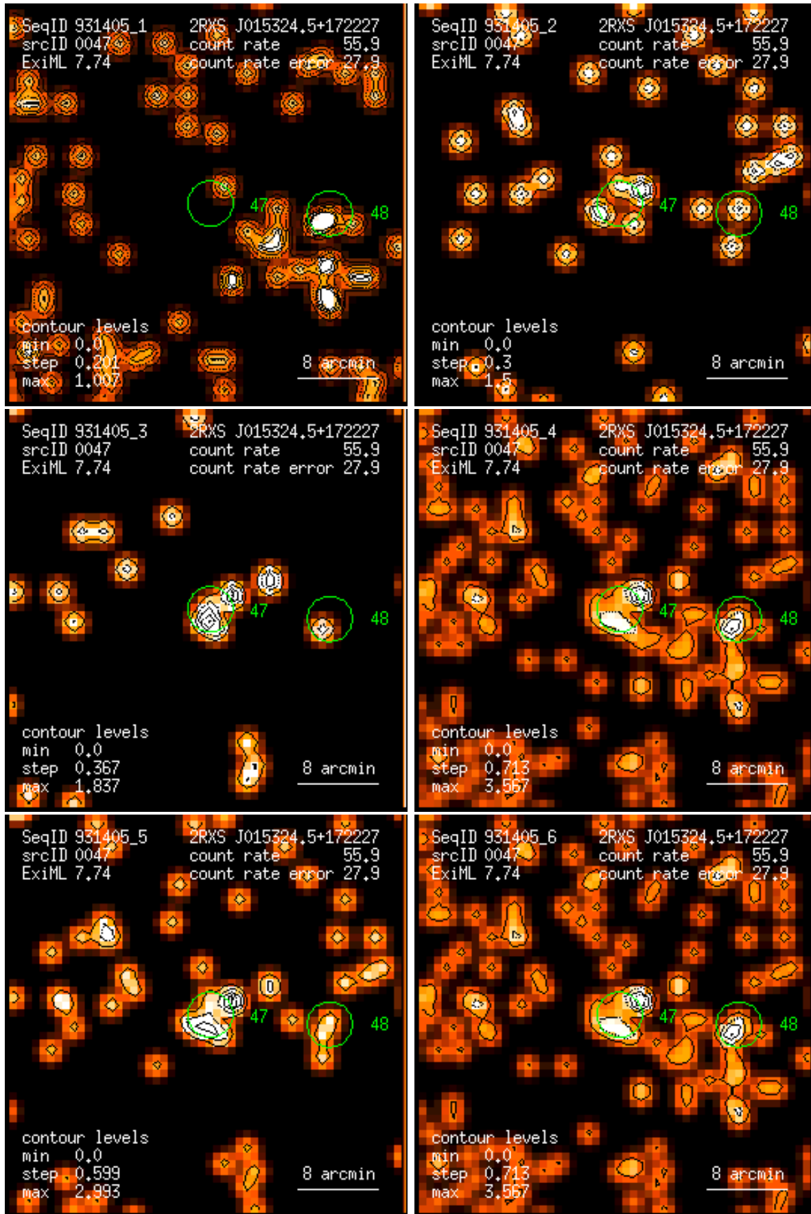
Figure 47: RASS 931405: detection 0047: band rate images, Gaussian filter: (1) PSPC channels 11 – 41, (2) 52 – 90, (3) 91 – 201, (4) 11 – 235, (5) 52 – 201, (6) 11 – 201. Broad band rates in counts/ks. Band rate contour levels in counts/ks/arcmin 2 .
