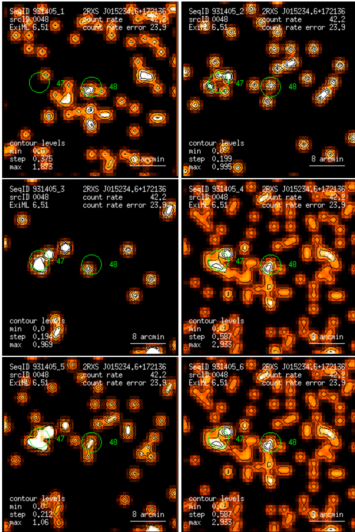
Figure 48: RASS 931405: detection 0048: band rate images, Gaussian filter: (1) PSPC channels 11 – 41, (2) 52 – 90, (3) 91 – 201, (4) 11 – 235, (5) 52 – 201, (6) 11 – 201. Broad band rates in counts/ks. Band rate contour levels in counts/ks/arcmin 2 .
