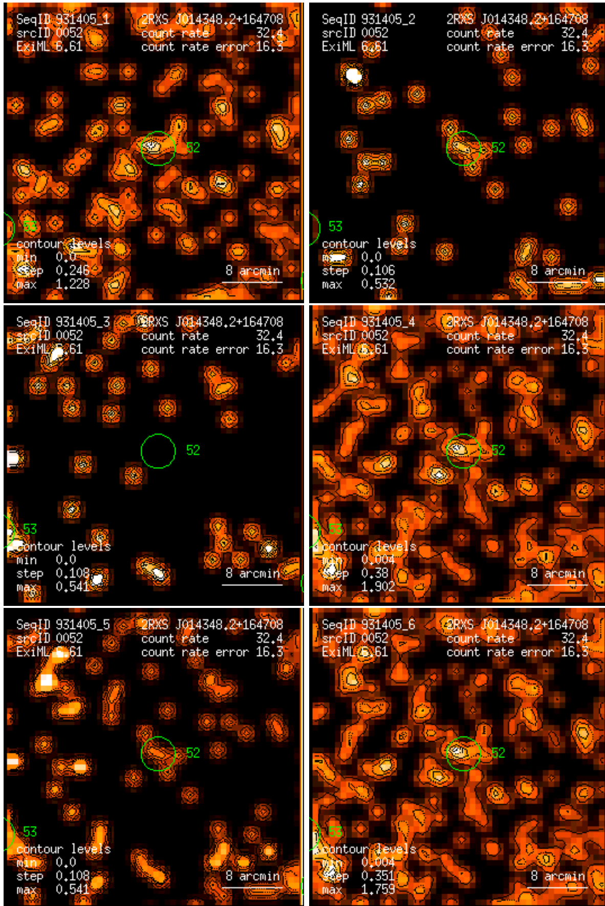
Figure 52: RASS 931405: detection 0052: band rate images, Gaussian filter: (1) PSPC channels 11 – 41, (2) 52 – 90, (3) 91 – 201, (4) 11 – 235, (5) 52 – 201, (6) 11 – 201. Broad band rates in counts/ks. Band rate contour levels in counts/ks/arcmin 2 .
