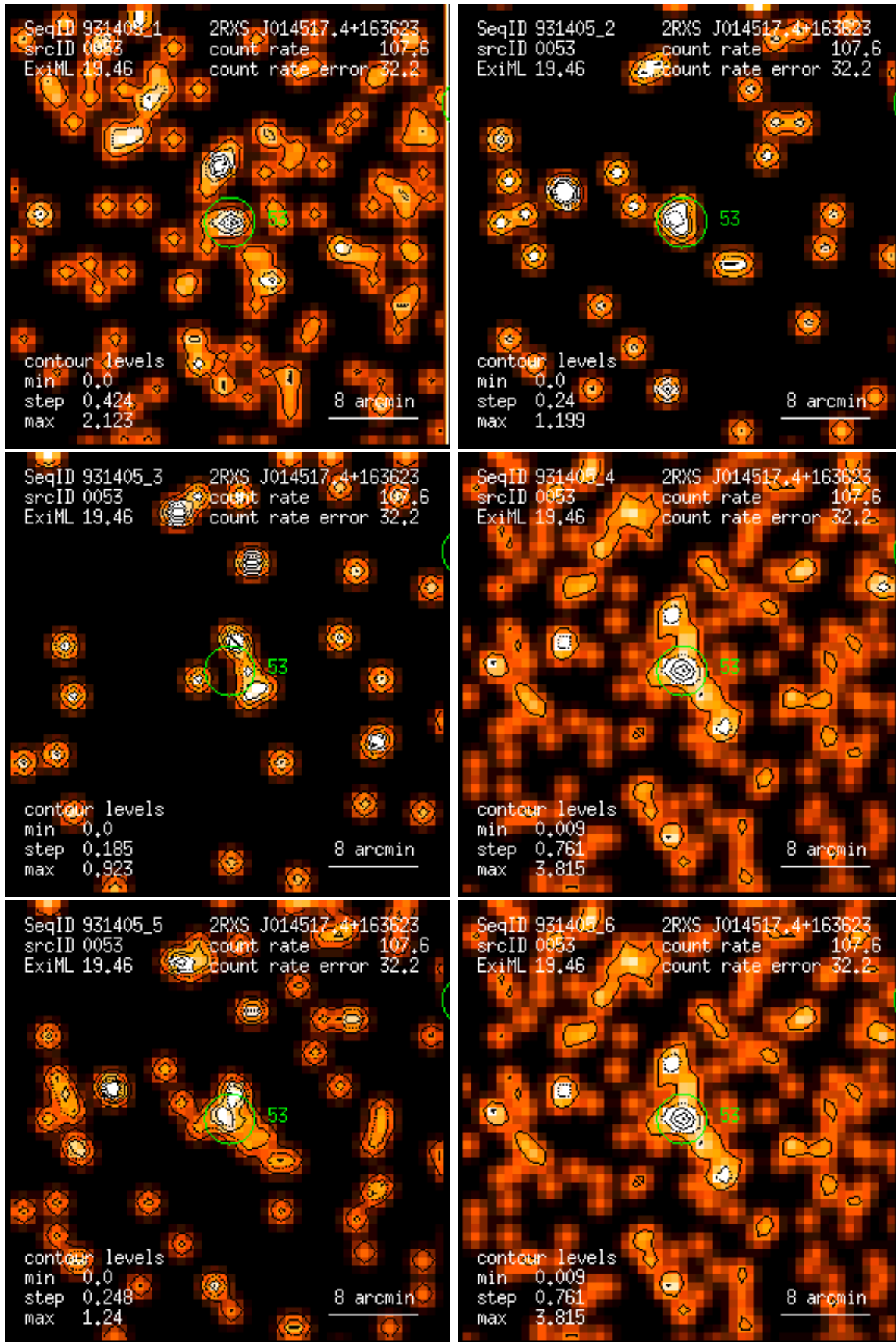
Figure 53: RASS 931405: detection 0053: band rate images, Gaussian filter: (1) PSPC channels 11 – 41, (2) 52 – 90, (3) 91 – 201, (4) 11 – 235, (5) 52 – 201, (6) 11 – 201. Broad band rates in counts/ks. Band rate contour levels in counts/ks/arcmin 2 .
