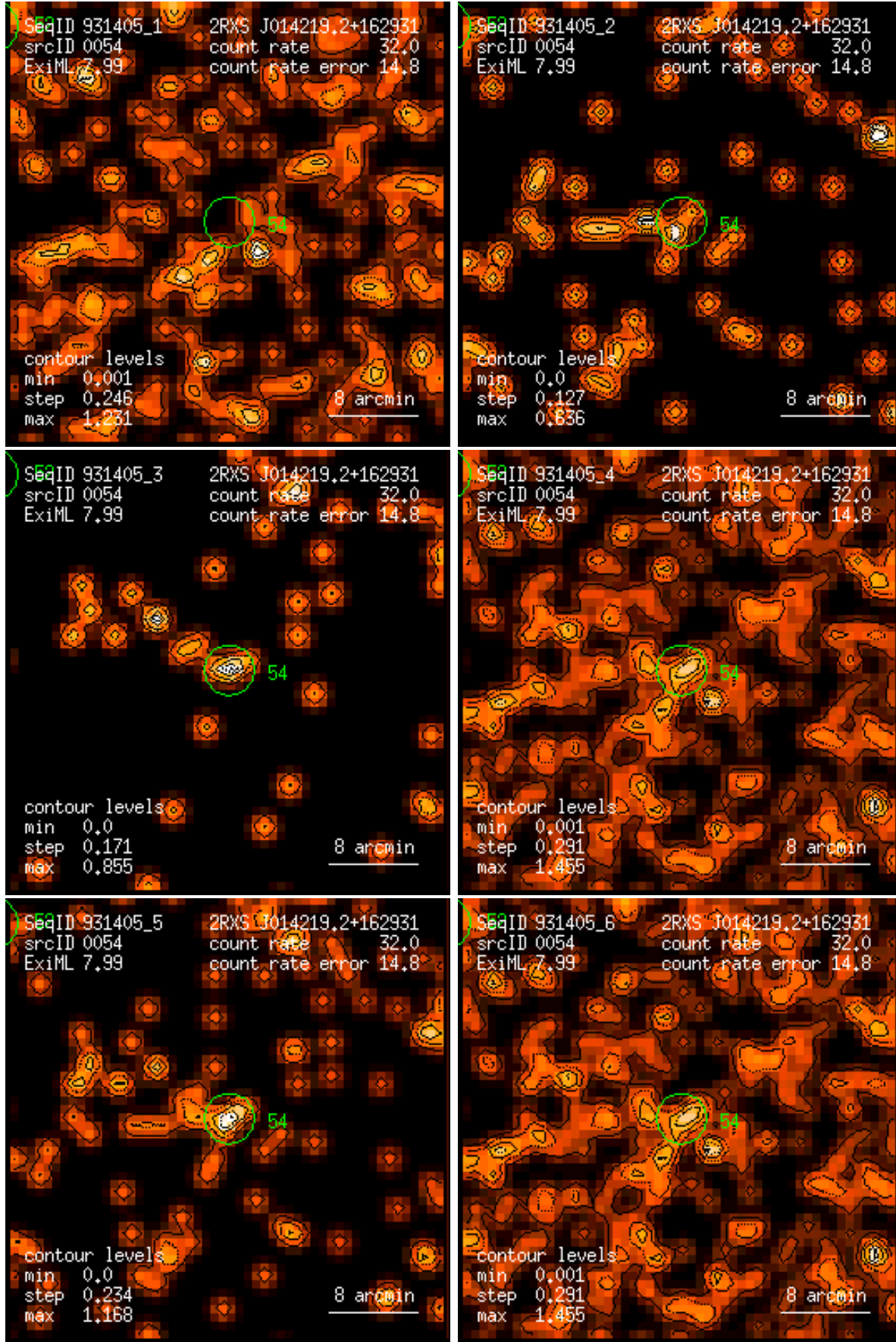
Figure 54: RASS 931405: detection 0054: band rate images, Gaussian filter: (1) PSPC channels 11 – 41, (2) 52 – 90, (3) 91 – 201, (4) 11 – 235, (5) 52 – 201, (6) 11 – 201. Broad band rates in counts/ks. Band rate contour levels in counts/ks/arcmin 2 .
