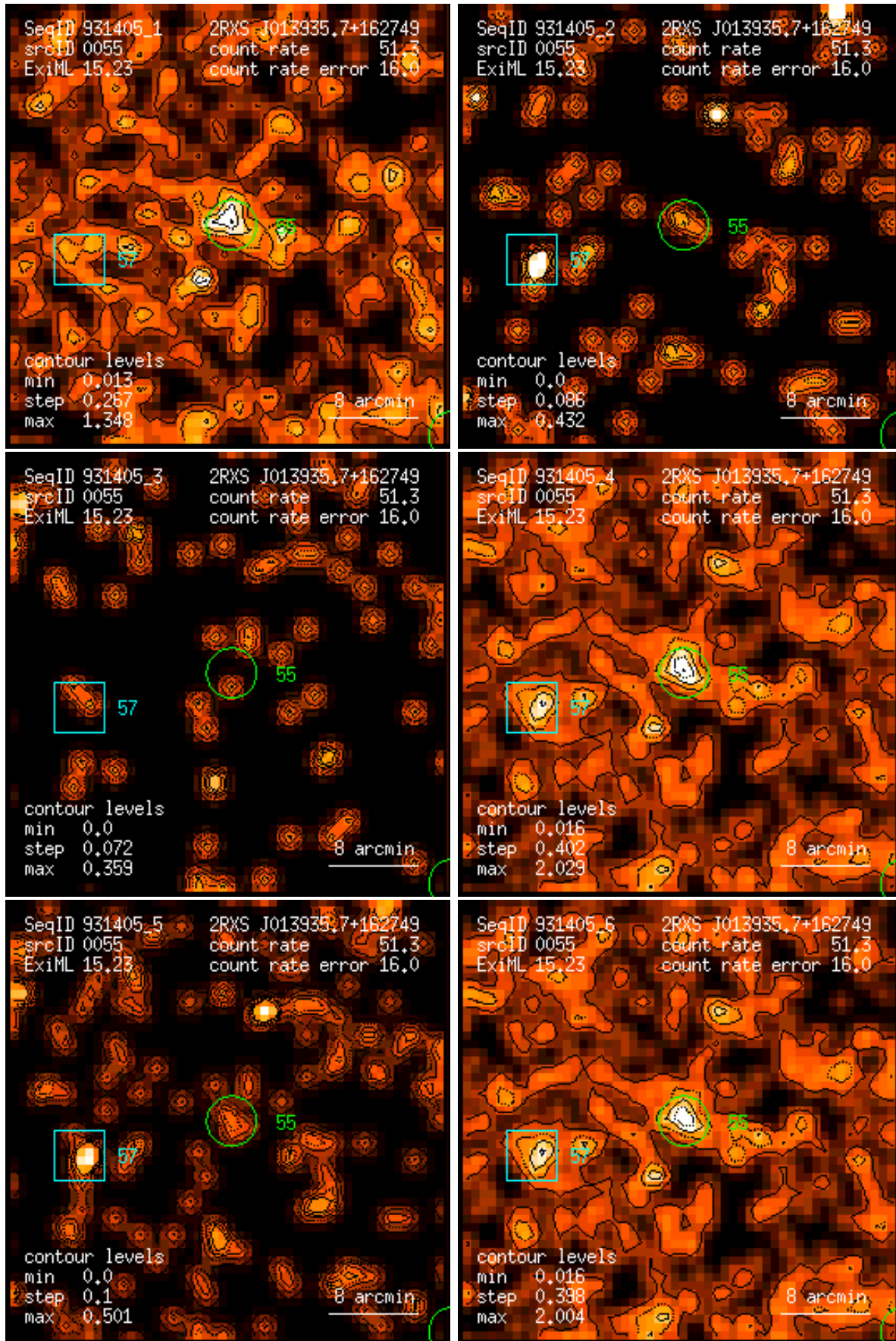
Figure 55: RASS 931405: detection 0055: band rate images, Gaussian filter: (1) PSPC channels 11 – 41, (2) 52 – 90, (3) 91 – 201, (4) 11 – 235, (5) 52 – 201, (6) 11 – 201. Broad band rates in counts/ks. Band rate contour levels in counts/ks/arcmin 2 .
