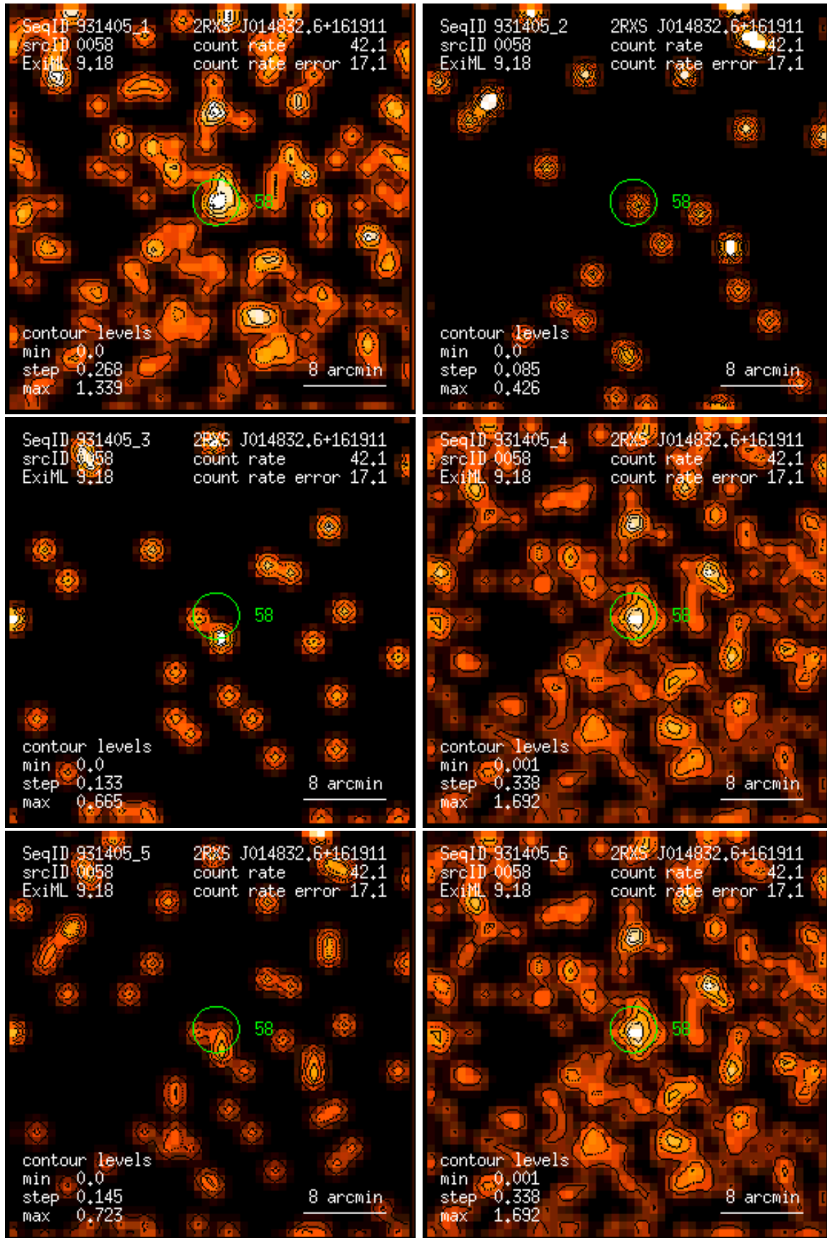
Figure 58: RASS 931405: detection 0058: band rate images, Gaussian filter: (1) PSPC channels 11 – 41, (2) 52 – 90, (3) 91 – 201, (4) 11 – 235, (5) 52 – 201, (6) 11 – 201. Broad band rates in counts/ks. Band rate contour levels in counts/ks/arcmin 2 .
