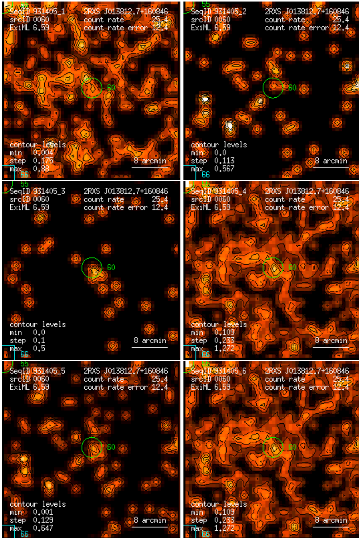
Figure 60: RASS 931405: detection 0060: band rate images, Gaussian filter: (1) PSPC channels 11 – 41, (2) 52 – 90, (3) 91 – 201, (4) 11 – 235, (5) 52 – 201, (6) 11 – 201. Broad band rates in counts/ks. Band rate contour levels in counts/ks/arcmin 2 .
