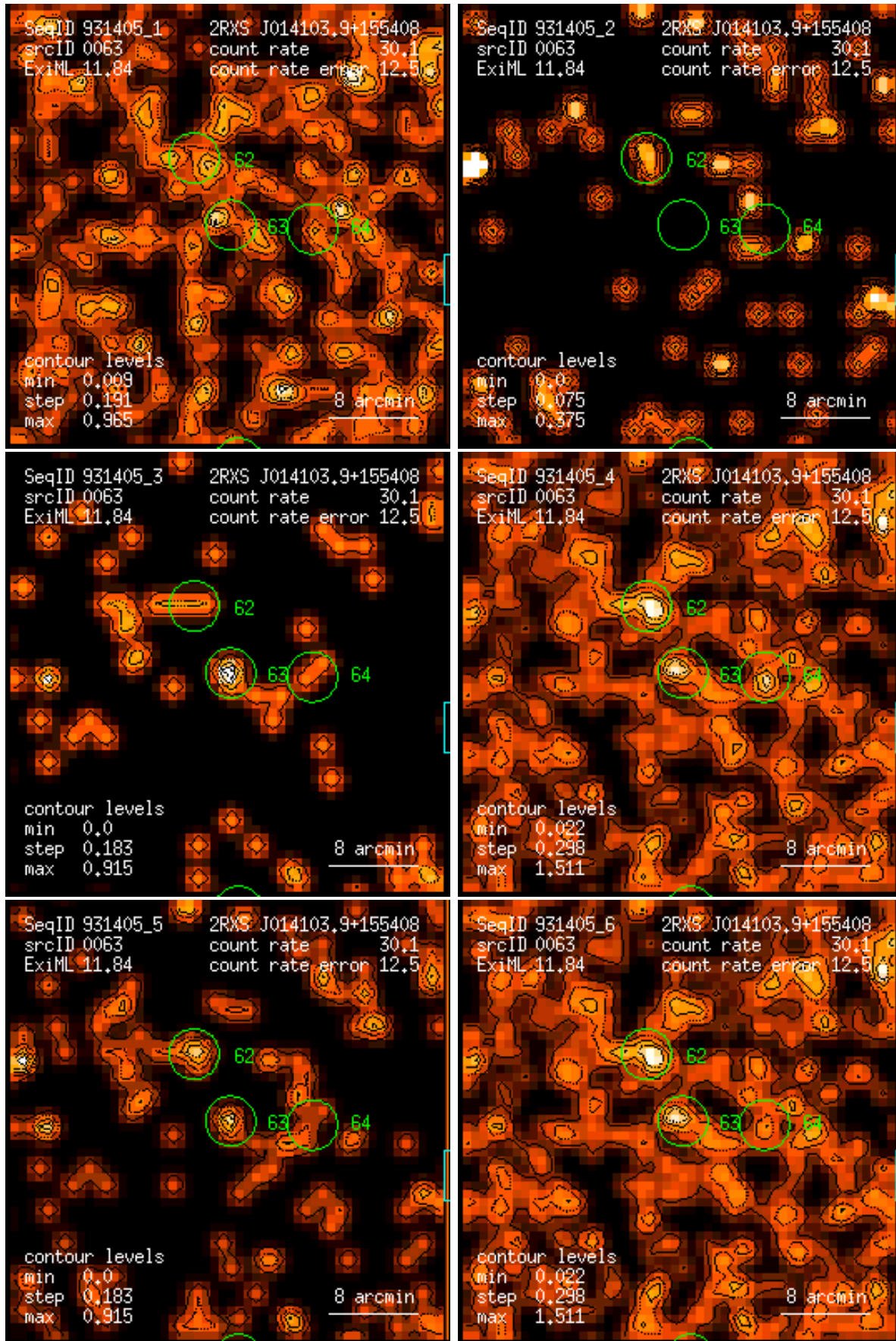
Figure 63: RASS 931405: detection 0063: band rate images, Gaussian filter: (1) PSPC channels 11 – 41, (2) 52 – 90, (3) 91 – 201, (4) 11 – 235, (5) 52 – 201, (6) 11 – 201. Broad band rates in counts/ks. Band rate contour levels in counts/ks/arcmin 2 .
