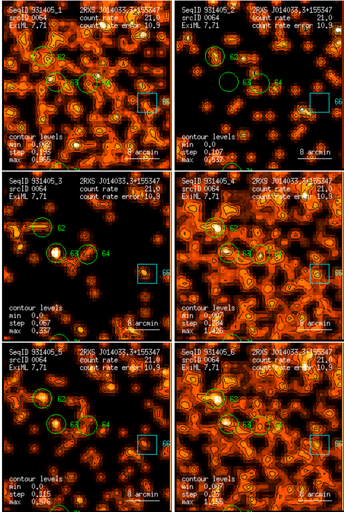
Figure 64: RASS 931405: detection 0064: band rate images, Gaussian filter: (1) PSPC channels 11 – 41, (2) 52 – 90, (3) 91 – 201, (4) 11 – 235, (5) 52 – 201, (6) 11 – 201. Broad band rates in counts/ks. Band rate contour levels in counts/ks/arcmin 2 .
