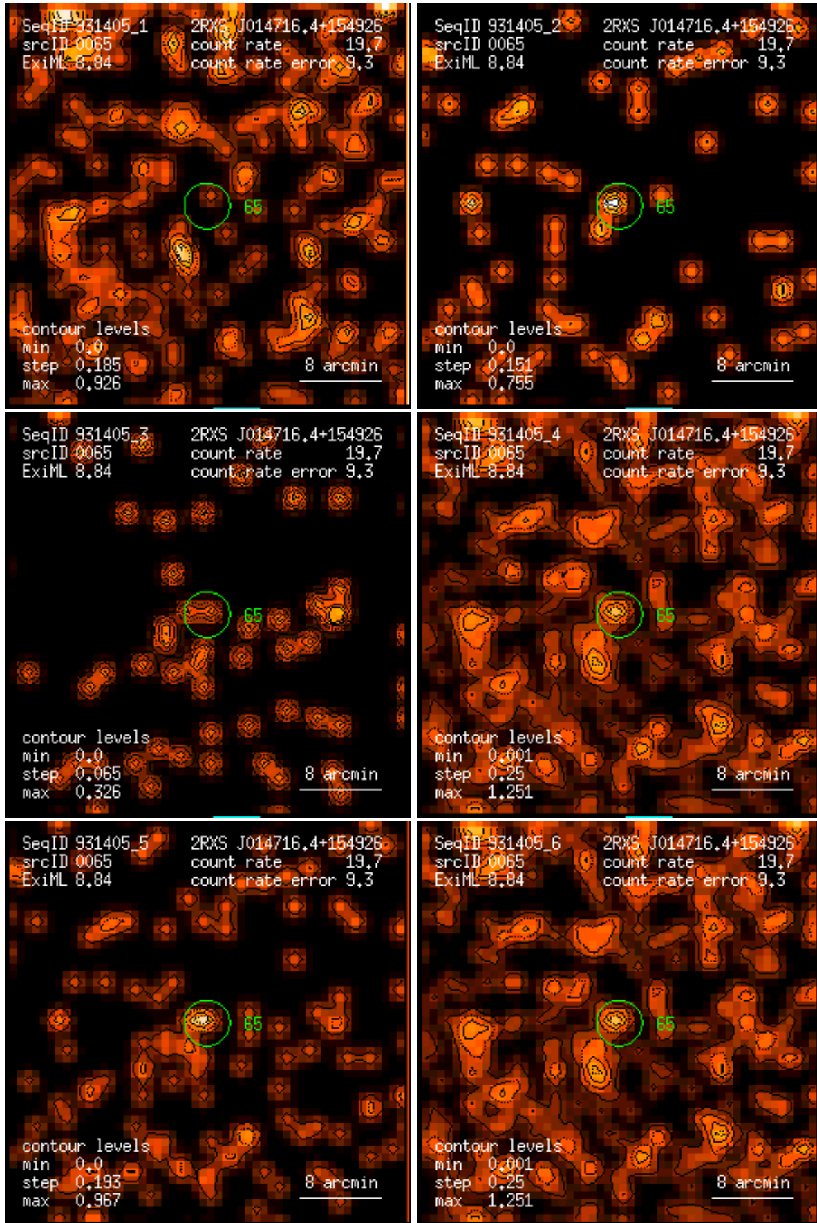
Figure 65: RASS 931405: detection 0065: band rate images, Gaussian filter: (1) PSPC channels 11 – 41, (2) 52 – 90, (3) 91 – 201, (4) 11 – 235, (5) 52 – 201, (6) 11 – 201. Broad band rates in counts/ks. Band rate contour levels in counts/ks/arcmin 2 .
