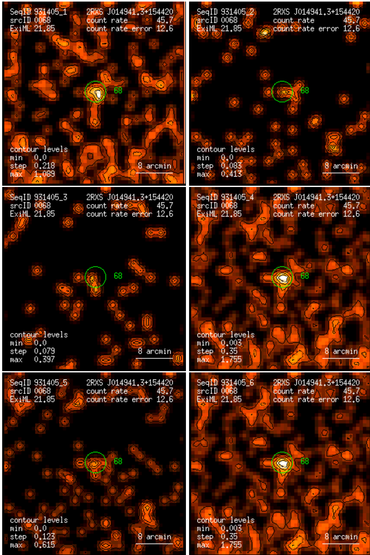
Figure 68: RASS 931405: detection 0068: band rate images, Gaussian filter: (1) PSPC channels 11 – 41, (2) 52 – 90, (3) 91 – 201, (4) 11 – 235, (5) 52 – 201, (6) 11 – 201. Broad band rates in counts/ks. Band rate contour levels in counts/ks/arcmin 2 .
