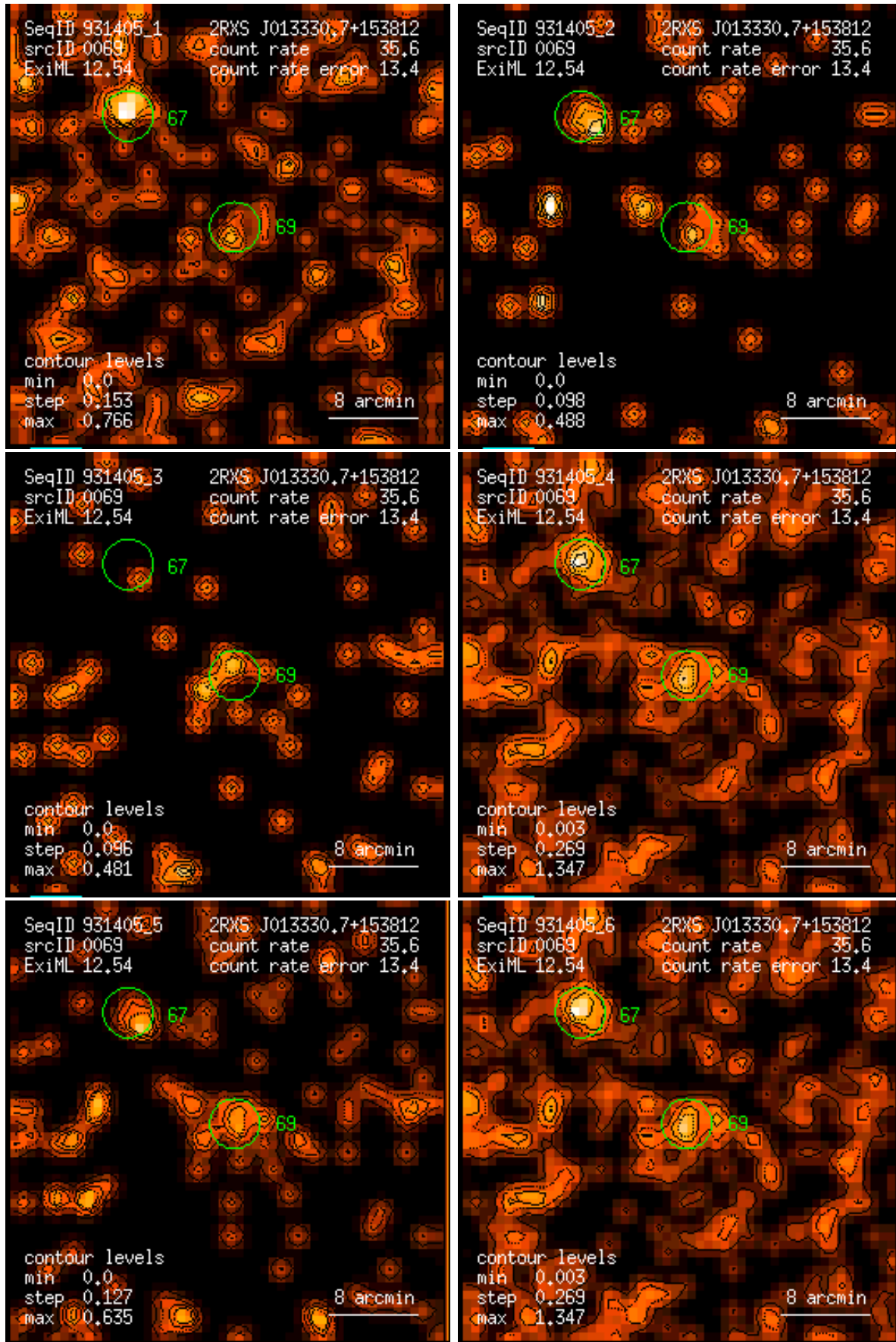
Figure 69: RASS 931405: detection 0069: band rate images, Gaussian filter: (1) PSPC channels 11 – 41, (2) 52 – 90, (3) 91 – 201, (4) 11 – 235, (5) 52 – 201, (6) 11 – 201. Broad band rates in counts/ks. Band rate contour levels in counts/ks/arcmin 2 .
