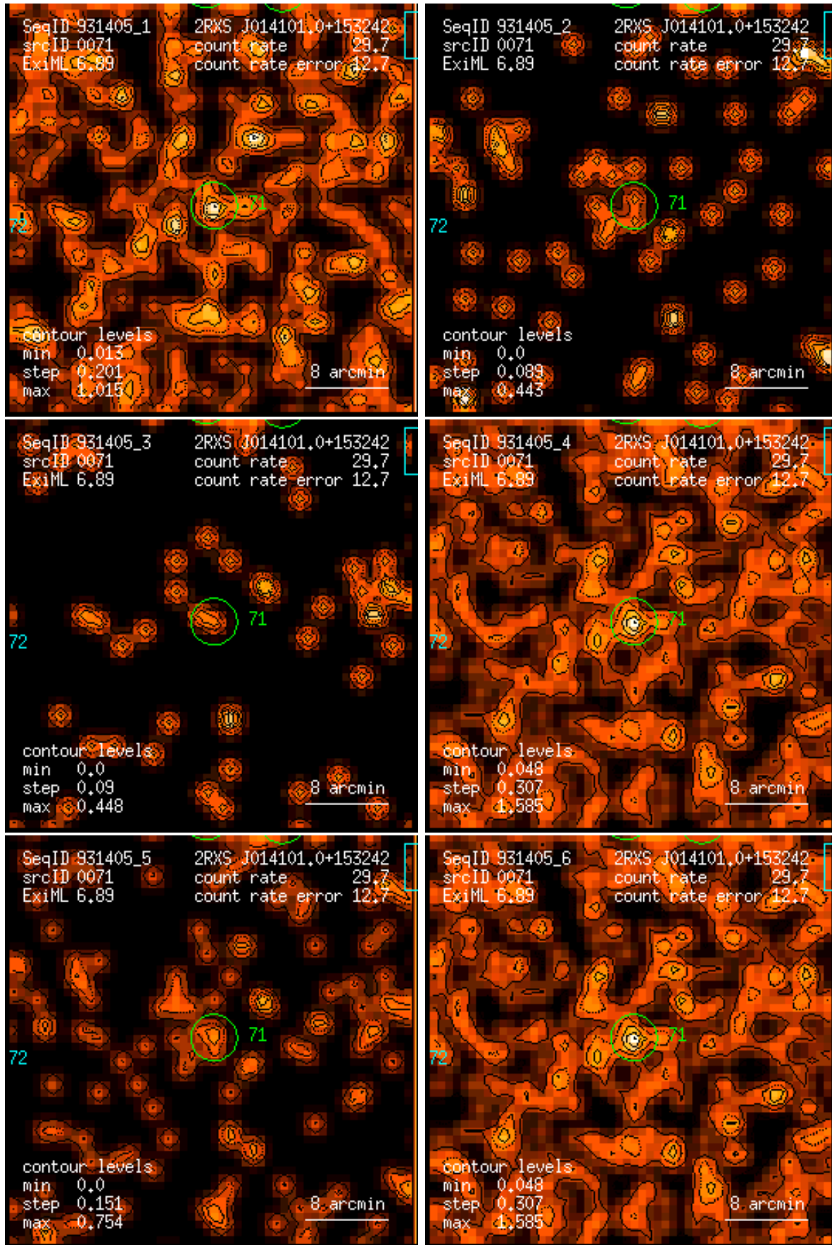
Figure 71: RASS 931405: detection 0071: band rate images, Gaussian filter: (1) PSPC channels 11 – 41, (2) 52 – 90, (3) 91 – 201, (4) 11 – 235, (5) 52 – 201, (6) 11 – 201. Broad band rates in counts/ks. Band rate contour levels in counts/ks/arcmin 2 .
