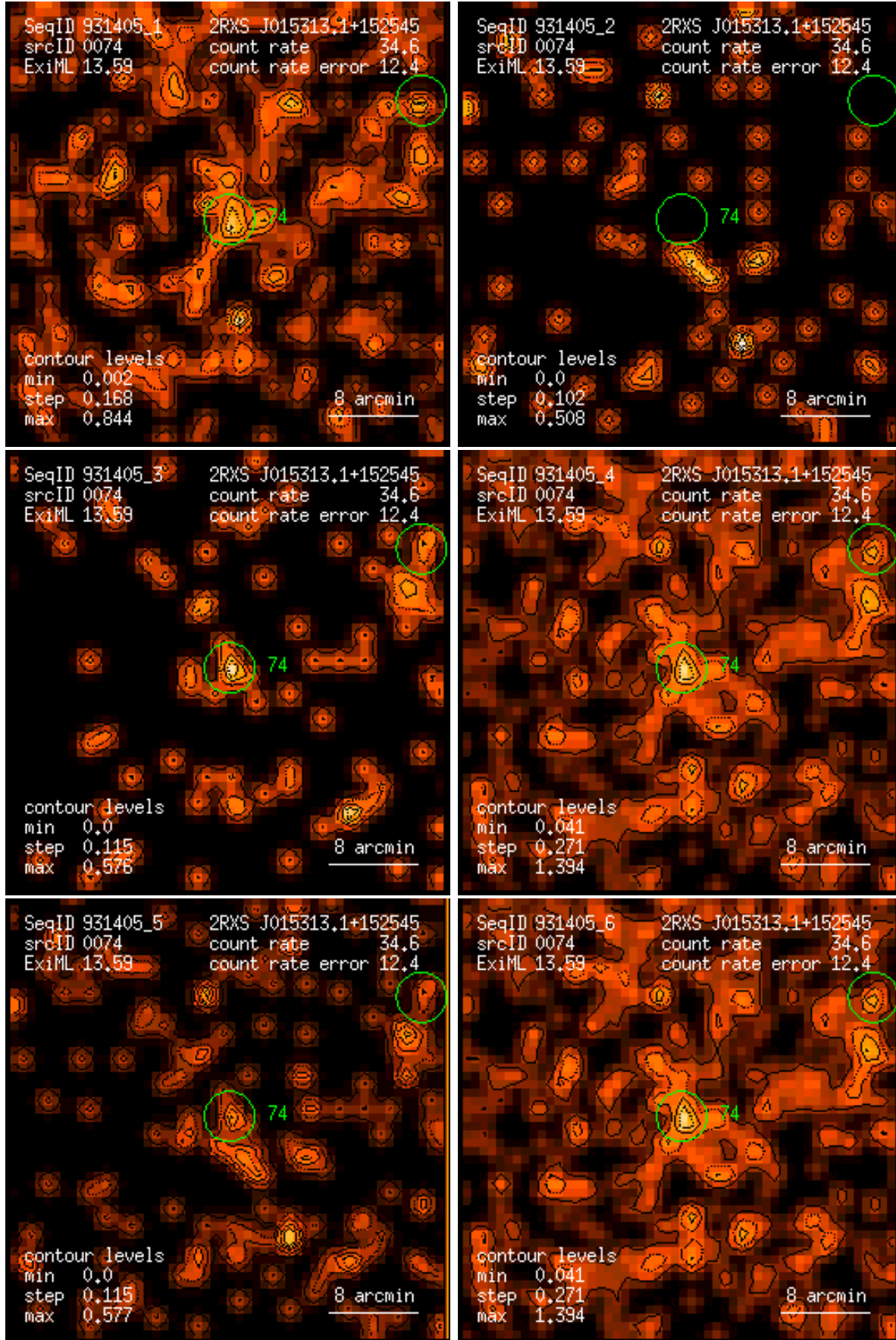
Figure 74: RASS 931405: detection 0074: band rate images, Gaussian filter: (1) PSPC channels 11 – 41, (2) 52 – 90, (3) 91 – 201, (4) 11 – 235, (5) 52 – 201, (6) 11 – 201. Broad band rates in counts/ks. Band rate contour levels in counts/ks/arcmin 2 .
