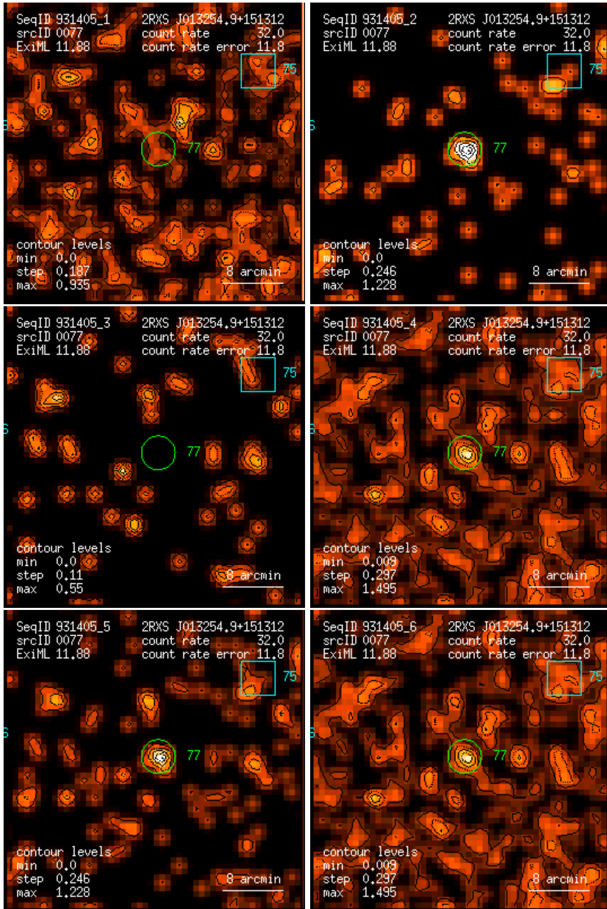
Figure 77: RASS 931405: detection 0077: band rate images, Gaussian filter: (1) PSPC channels 11 – 41, (2) 52 – 90, (3) 91 – 201, (4) 11 – 235, (5) 52 – 201, (6) 11 – 201. Broad band rates in counts/ks. Band rate contour levels in counts/ks/arcmin 2 .
