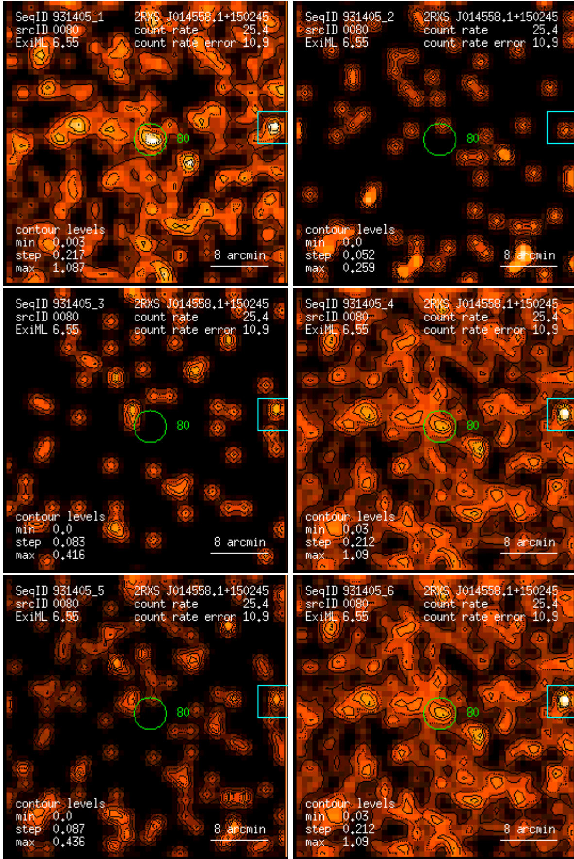
Figure 80: RASS 931405: detection 0080: band rate images, Gaussian filter: (1) PSPC channels 11 – 41, (2) 52 – 90, (3) 91 – 201, (4) 11 – 235, (5) 52 – 201, (6) 11 – 201. Broad band rates in counts/ks. Band rate contour levels in counts/ks/arcmin 2 .
