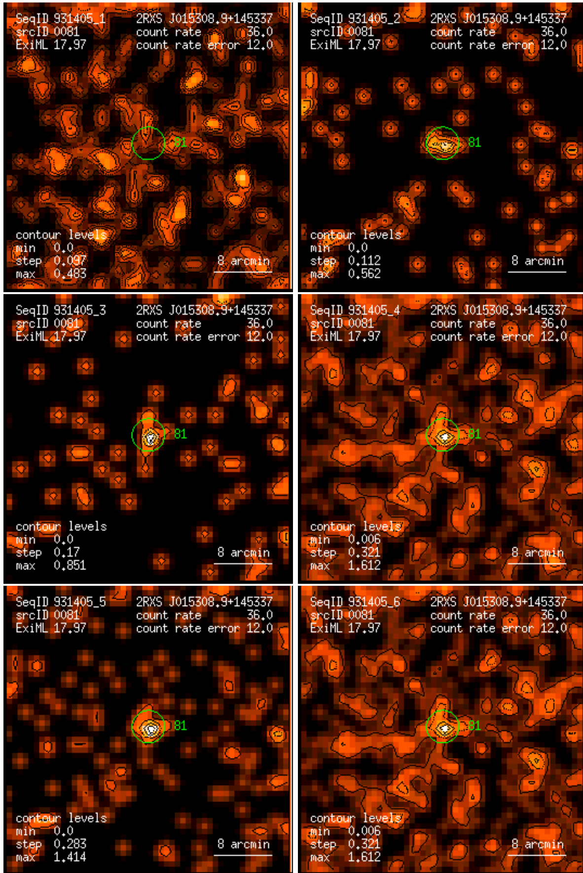
Figure 81: RASS 931405: detection 0081: band rate images, Gaussian filter: (1) PSPC channels 11 – 41, (2) 52 – 90, (3) 91 – 201, (4) 11 – 235, (5) 52 – 201, (6) 11 – 201. Broad band rates in counts/ks. Band rate contour levels in counts/ks/arcmin 2 .
