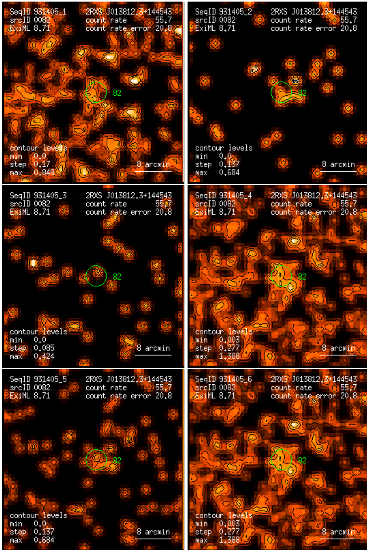
Figure 82: RASS 931405: detection 0082: band rate images, Gaussian filter: (1) PSPC channels 11 – 41, (2) 52 – 90, (3) 91 – 201, (4) 11 – 235, (5) 52 – 201, (6) 11 – 201. Broad band rates in counts/ks. Band rate contour levels in counts/ks/arcmin 2 .
