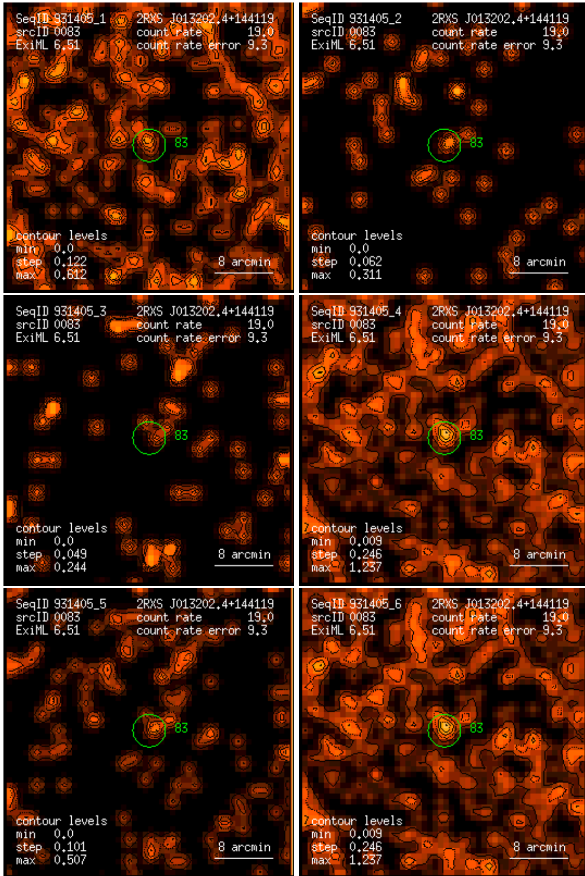
Figure 83: RASS 931405: detection 0083: band rate images, Gaussian filter: (1) PSPC channels 11 – 41, (2) 52 – 90, (3) 91 – 201, (4) 11 – 235, (5) 52 – 201, (6) 11 – 201. Broad band rates in counts/ks. Band rate contour levels in counts/ks/arcmin 2 .
