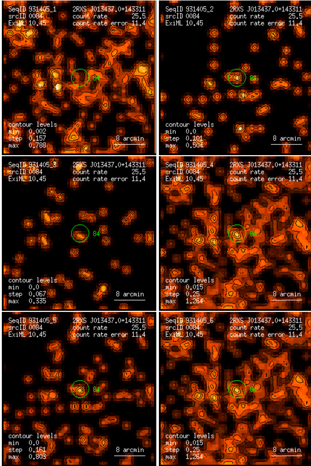
Figure 84: RASS 931405: detection 0084: band rate images, Gaussian filter: (1) PSPC channels 11 – 41, (2) 52 – 90, (3) 91 – 201, (4) 11 – 235, (5) 52 – 201, (6) 11 – 201. Broad band rates in counts/ks. Band rate contour levels in counts/ks/arcmin 2 .
