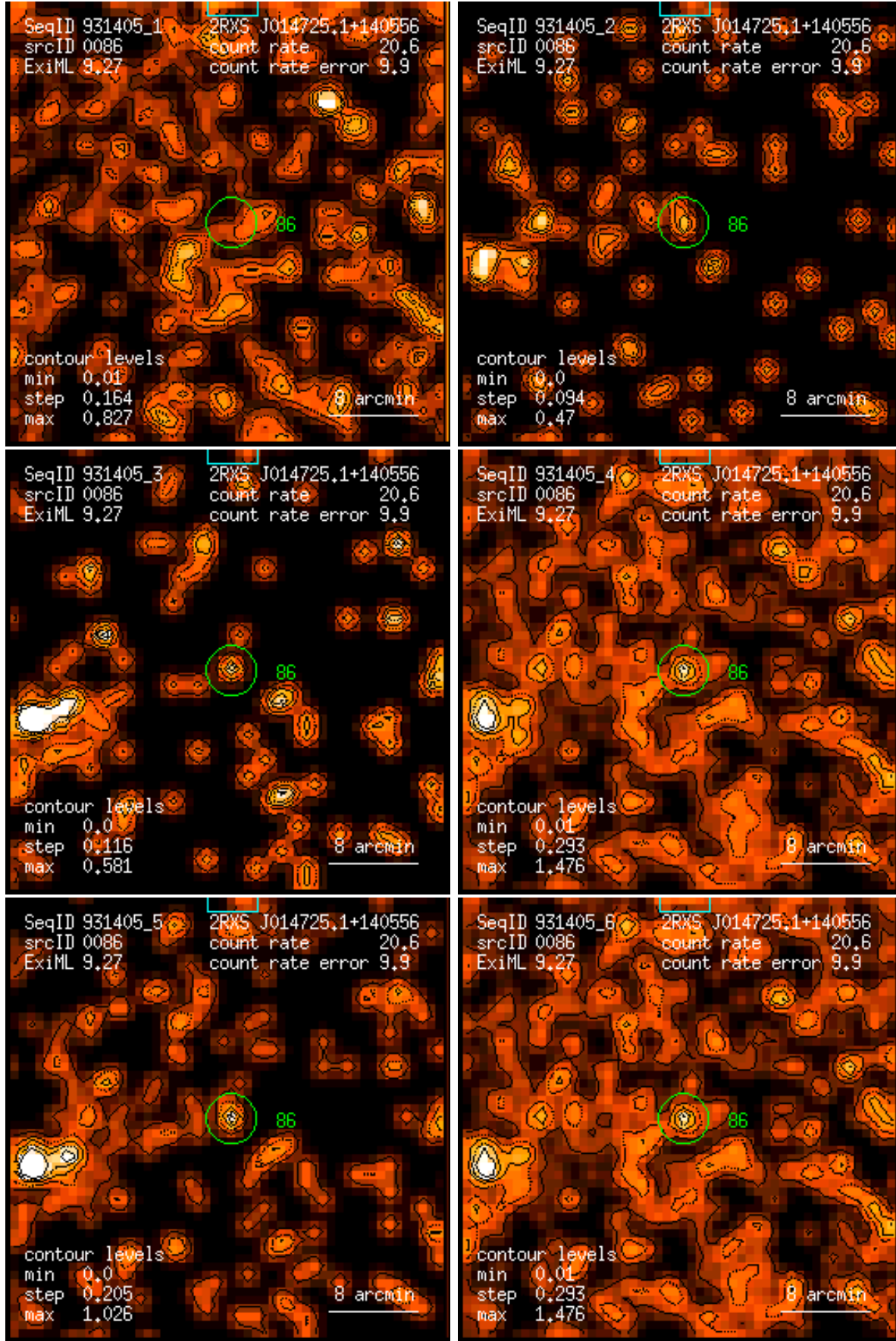
Figure 86: RASS 931405: detection 0086: band rate images, Gaussian filter: (1) PSPC channels 11 – 41, (2) 52 – 90, (3) 91 – 201, (4) 11 – 235, (5) 52 – 201, (6) 11 – 201. Broad band rates in counts/ks. Band rate contour levels in counts/ks/arcmin 2 .
