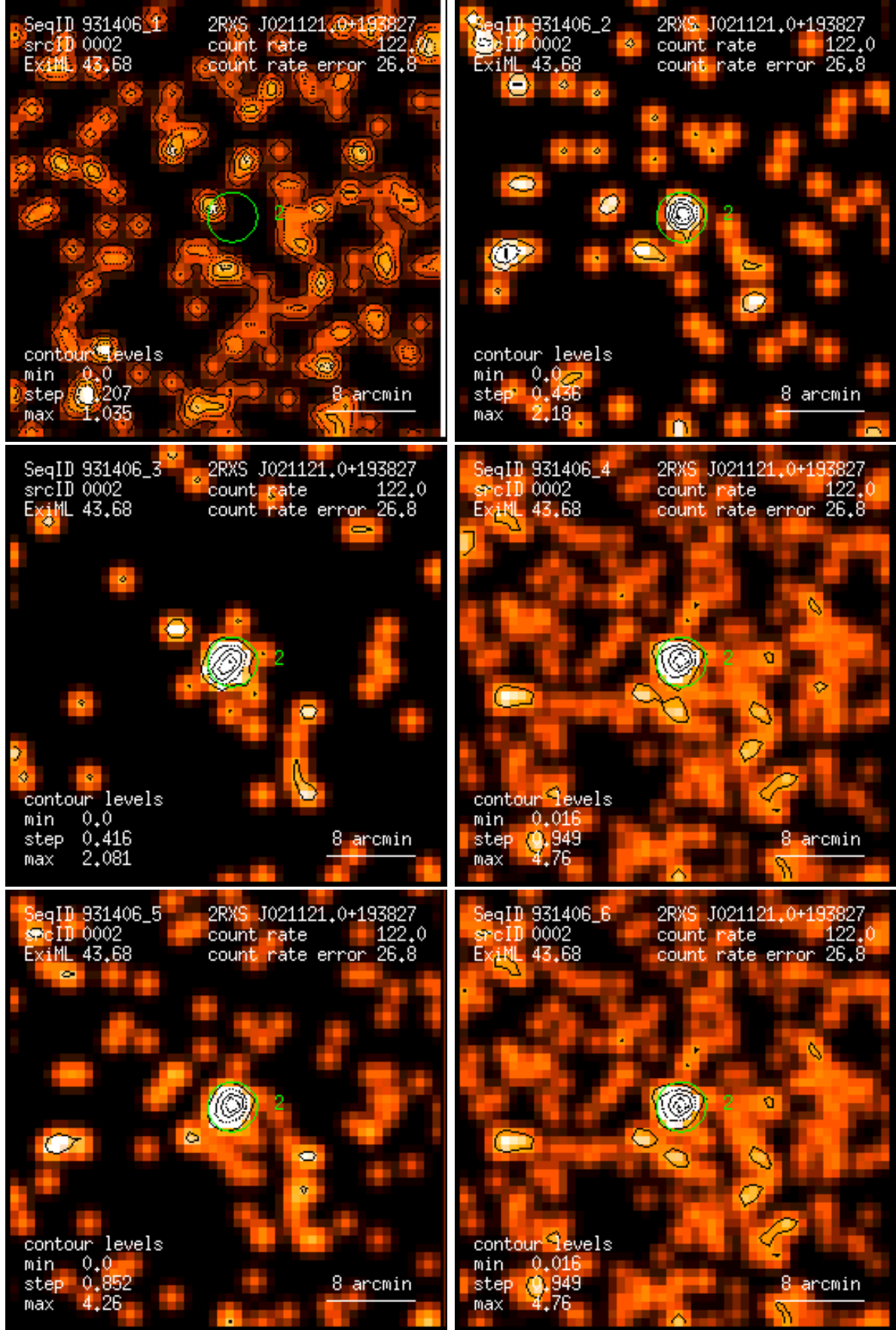
Figure 2: RASS 931406: detection 0002: band rate images, Gaussian filter: (1) PSPC channels 11 – 41, (2) 52 – 90, (3) 91 – 201, (4) 11 – 235, (5) 52 – 201, (6) 11 – 201. Broad band rates in counts/ks. Band rate contour levels in counts/ks/arcmin 2 .
