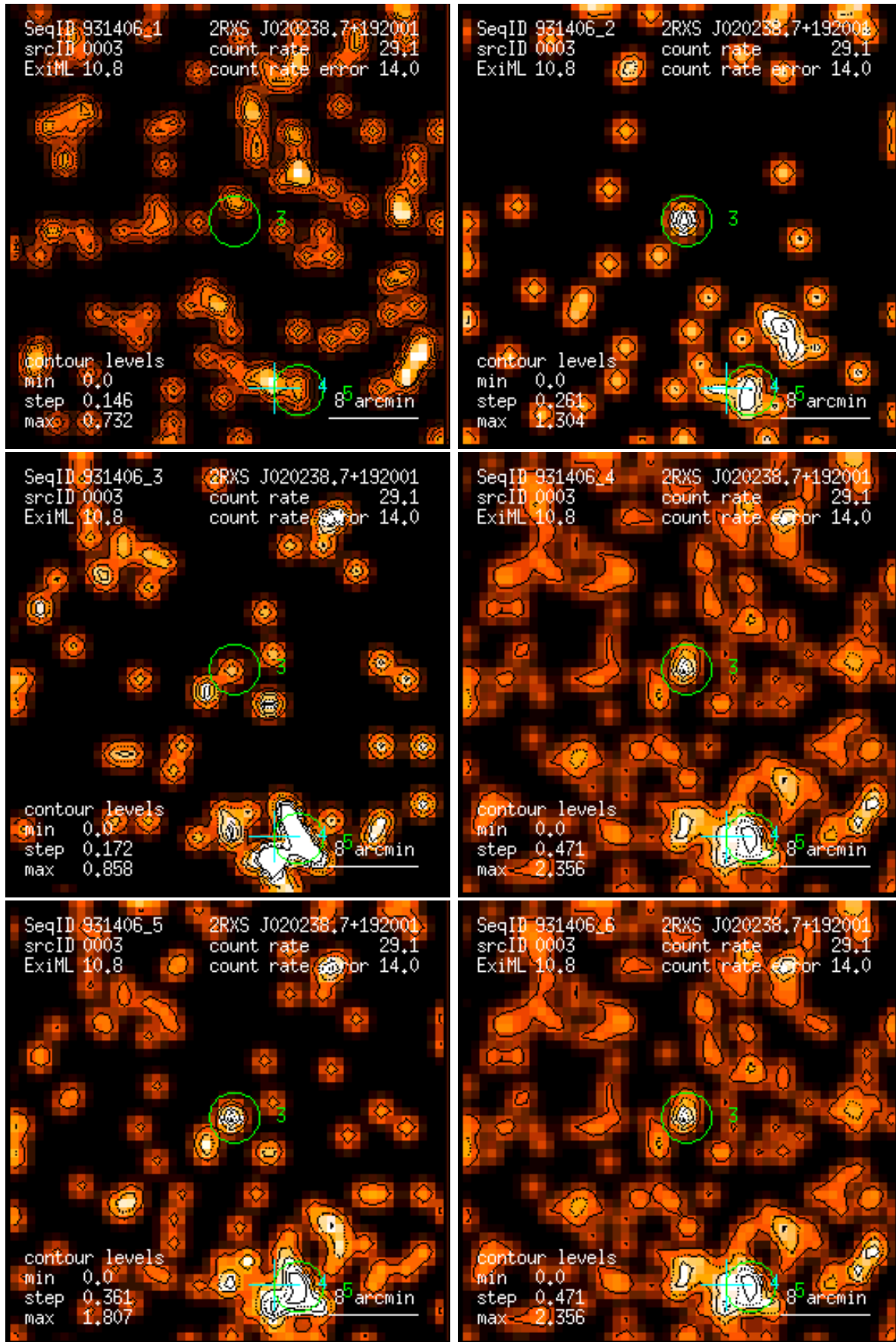
Figure 3: RASS 931406: detection 0003: band rate images, Gaussian filter: (1) PSPC channels 11 – 41, (2) 52 – 90, (3) 91 – 201, (4) 11 – 235, (5) 52 – 201, (6) 11 – 201. Broad band rates in counts/ks. Band rate contour levels in counts/ks/arcmin 2 .
