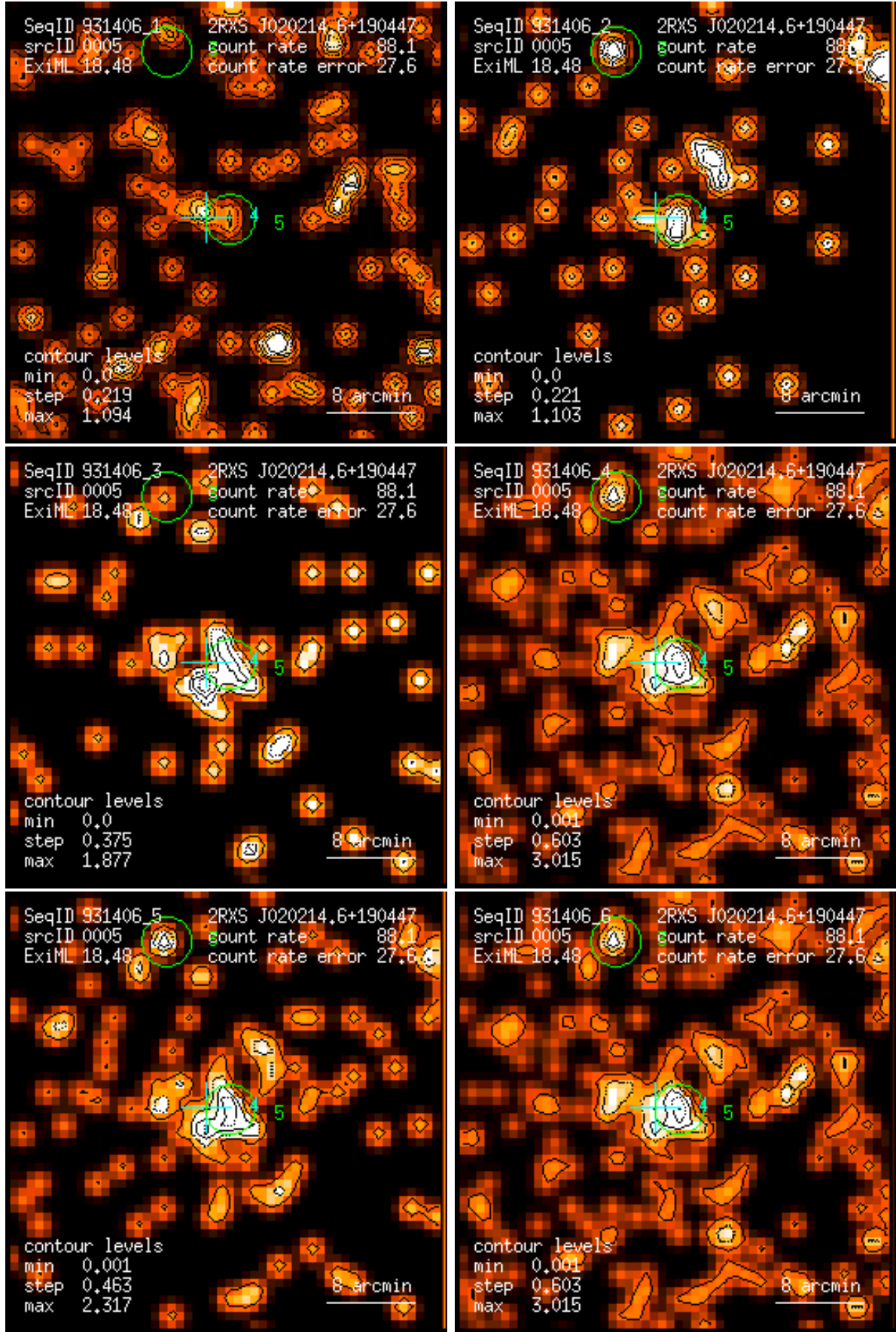
Figure 5: RASS 931406: detection 0005: band rate images, Gaussian filter: (1) PSPC channels 11 – 41, (2) 52 – 90, (3) 91 – 201, (4) 11 – 235, (5) 52 – 201, (6) 11 – 201. Broad band rates in counts/ks. Band rate contour levels in counts/ks/arcmin 2 .
