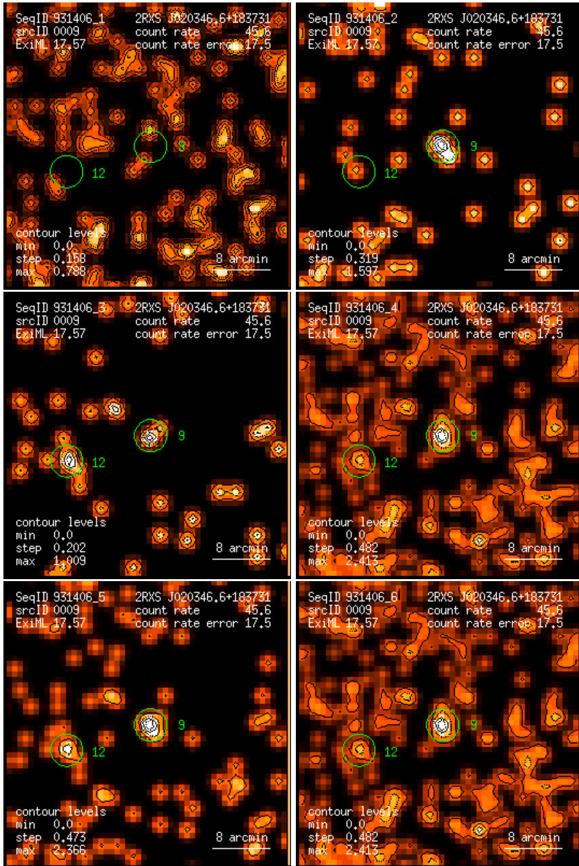
Figure 9: RASS 931406: detection 0009: band rate images, Gaussian filter: (1) PSPC channels 11 – 41, (2) 52 – 90, (3) 91 – 201, (4) 11 – 235, (5) 52 – 201, (6) 11 – 201. Broad band rates in counts/ks. Band rate contour levels in counts/ks/arcmin 2 .
