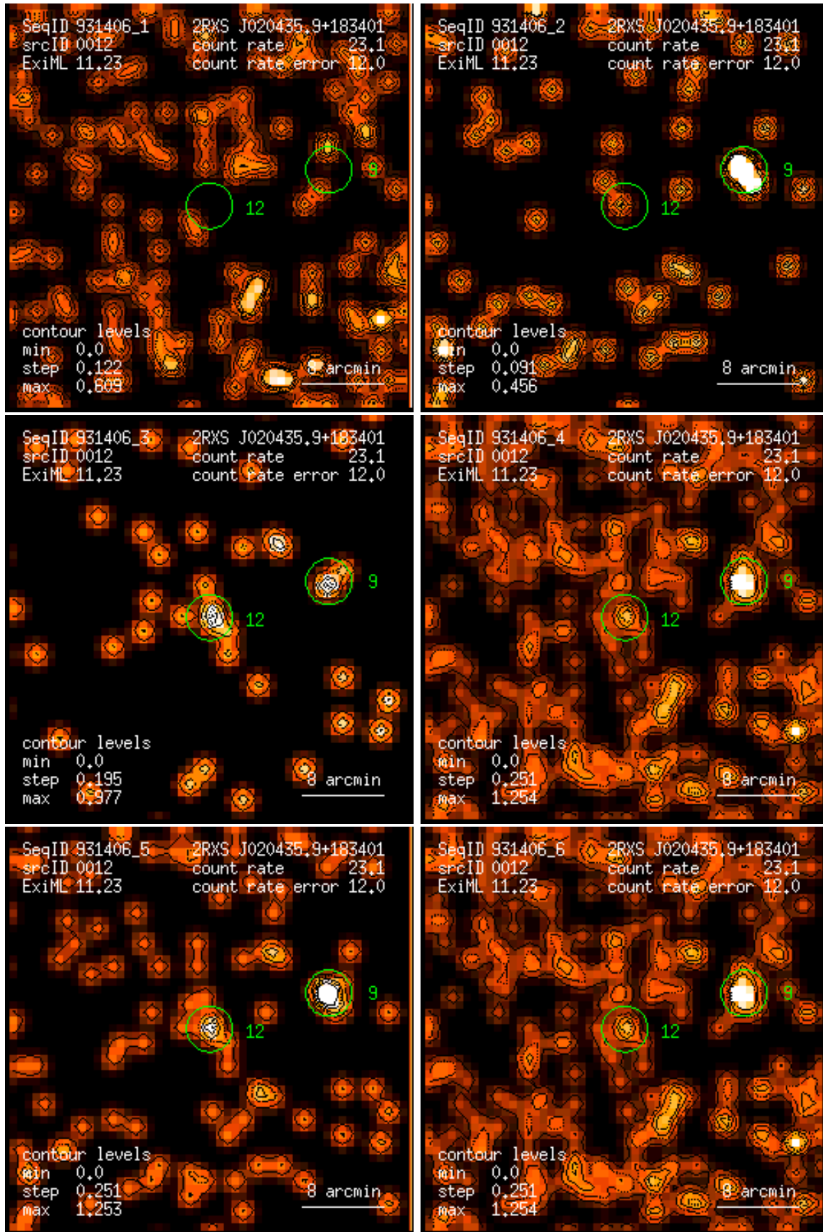
Figure 12: RASS 931406: detection 0012: band rate images, Gaussian filter: (1) PSPC channels 11 – 41, (2) 52 – 90, (3) 91 – 201, (4) 11 – 235, (5) 52 – 201, (6) 11 – 201. Broad band rates in counts/ks. Band rate contour levels in counts/ks/arcmin 2 .
