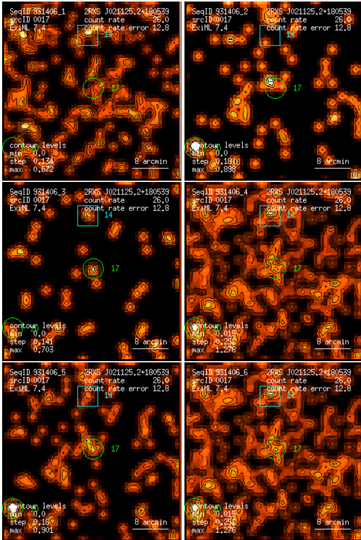
Figure 17: RASS 931406: detection 0017: band rate images, Gaussian filter: (1) PSPC channels 11 – 41, (2) 52 – 90, (3) 91 – 201, (4) 11 – 235, (5) 52 – 201, (6) 11 – 201. Broad band rates in counts/ks. Band rate contour levels in counts/ks/arcmin 2 .
