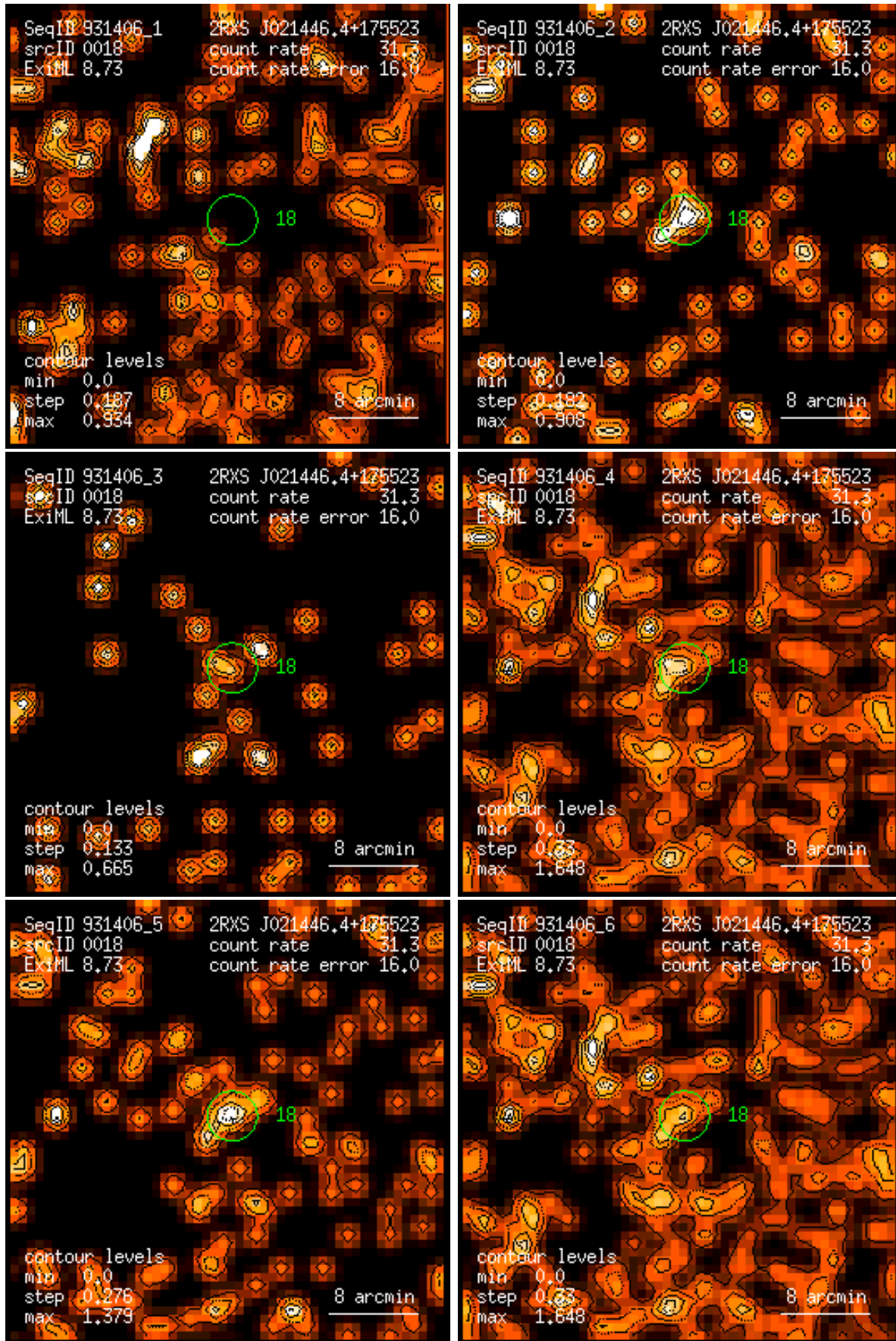
Figure 18: RASS 931406: detection 0018: band rate images, Gaussian filter: (1) PSPC channels 11 – 41, (2) 52 – 90, (3) 91 – 201, (4) 11 – 235, (5) 52 – 201, (6) 11 – 201. Broad band rates in counts/ks. Band rate contour levels in counts/ks/arcmin 2 .
