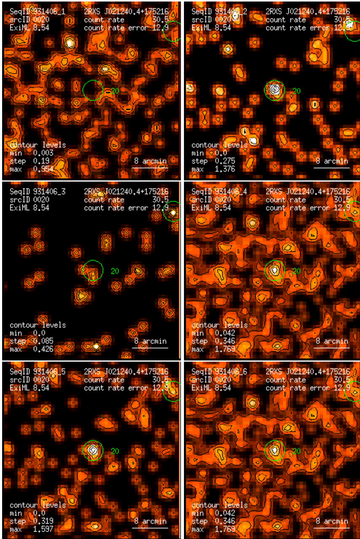
Figure 20: RASS 931406: detection 0020: band rate images, Gaussian filter: (1) PSPC channels 11 – 41, (2) 52 – 90, (3) 91 – 201, (4) 11 – 235, (5) 52 – 201, (6) 11 – 201. Broad band rates in counts/ks. Band rate contour levels in counts/ks/arcmin 2 .
