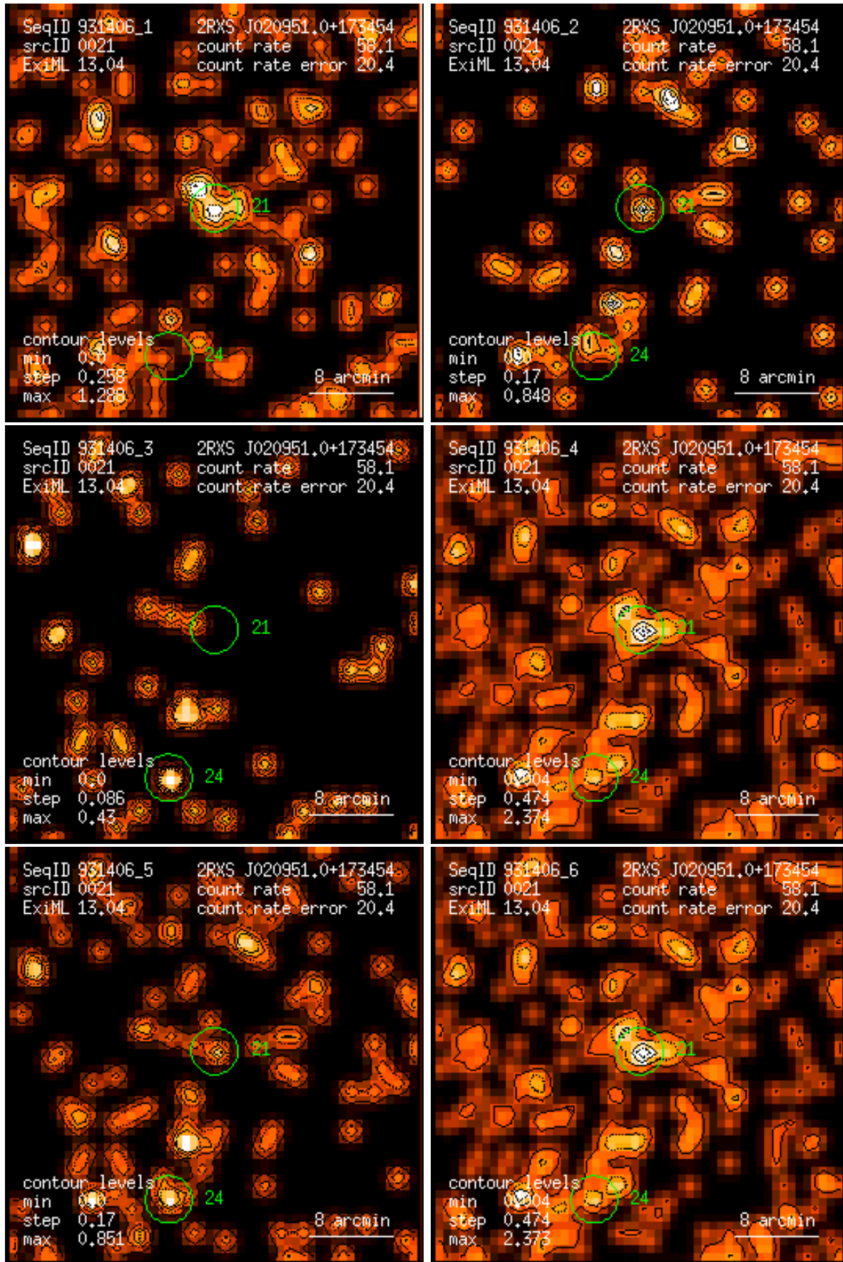
Figure 21: RASS 931406: detection 0021: band rate images, Gaussian filter: (1) PSPC channels 11 – 41, (2) 52 – 90, (3) 91 – 201, (4) 11 – 235, (5) 52 – 201, (6) 11 – 201. Broad band rates in counts/ks. Band rate contour levels in counts/ks/arcmin 2 .
