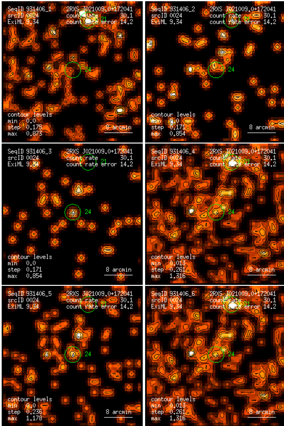
Figure 24: RASS 931406: detection 0024: band rate images, Gaussian filter: (1) PSPC channels 11 – 41, (2) 52 – 90, (3) 91 – 201, (4) 11 – 235, (5) 52 – 201, (6) 11 – 201. Broad band rates in counts/ks. Band rate contour levels in counts/ks/arcmin 2 .
