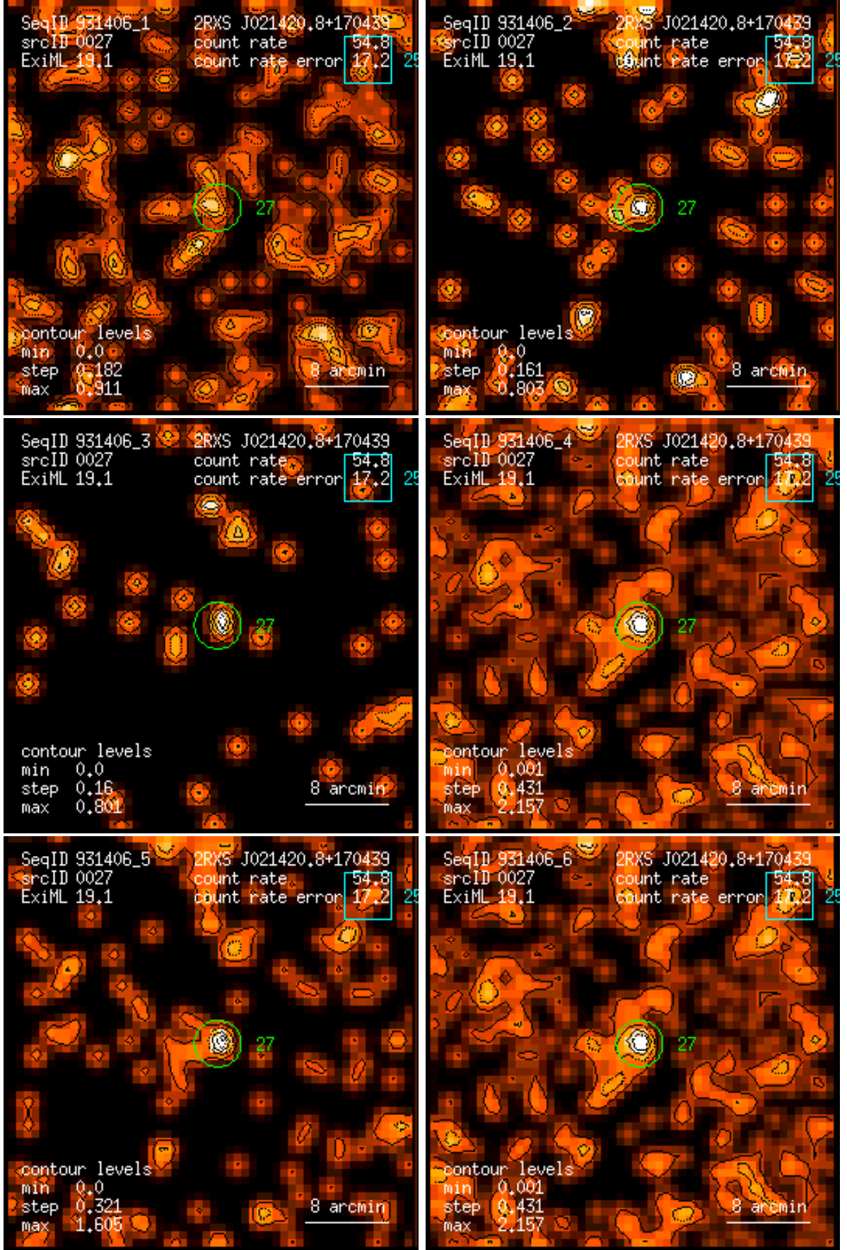
Figure 27: RASS 931406: detection 0027: band rate images, Gaussian filter: (1) PSPC channels 11 – 41, (2) 52 – 90, (3) 91 – 201, (4) 11 – 235, (5) 52 – 201, (6) 11 – 201. Broad band rates in counts/ks. Band rate contour levels in counts/ks/arcmin 2 .
