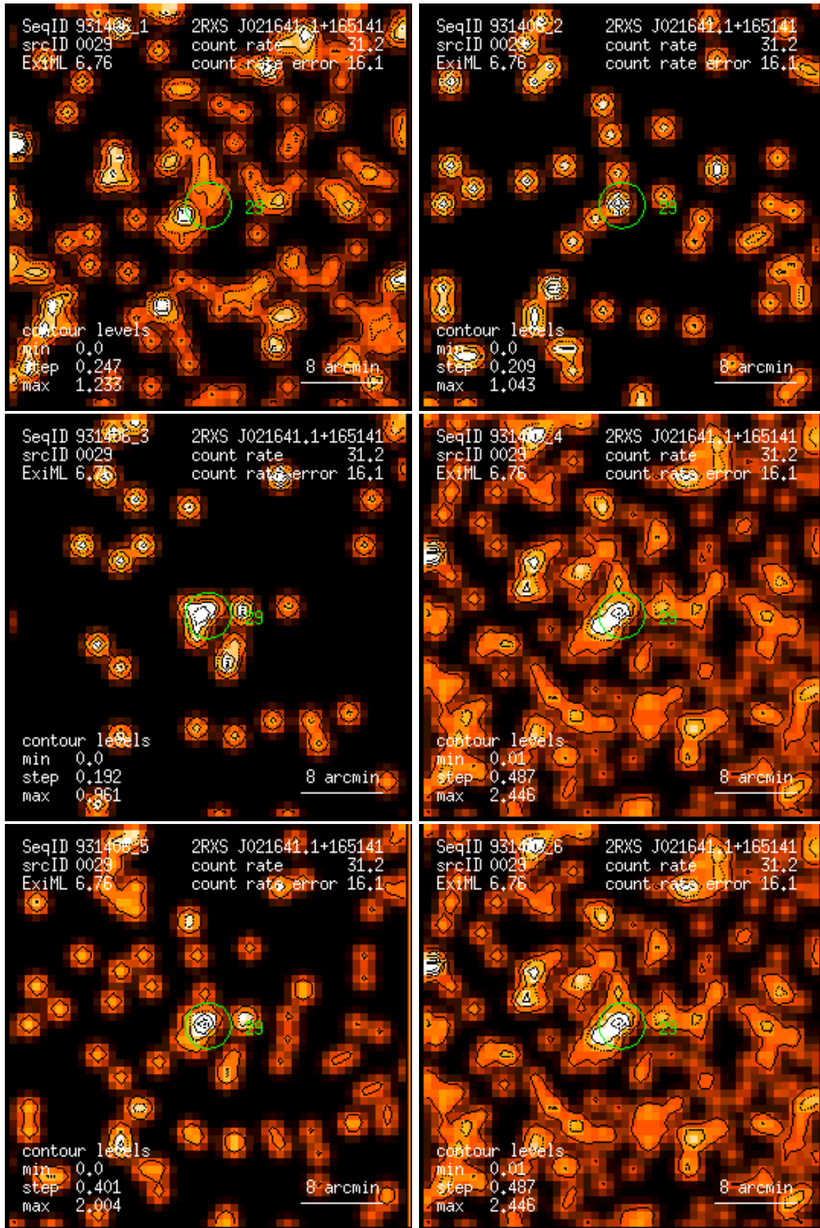
Figure 29: RASS 931406: detection 0029: band rate images, Gaussian filter: (1) PSPC channels 11 – 41, (2) 52 – 90, (3) 91 – 201, (4) 11 – 235, (5) 52 – 201, (6) 11 – 201. Broad band rates in counts/ks. Band rate contour levels in counts/ks/arcmin 2 .
