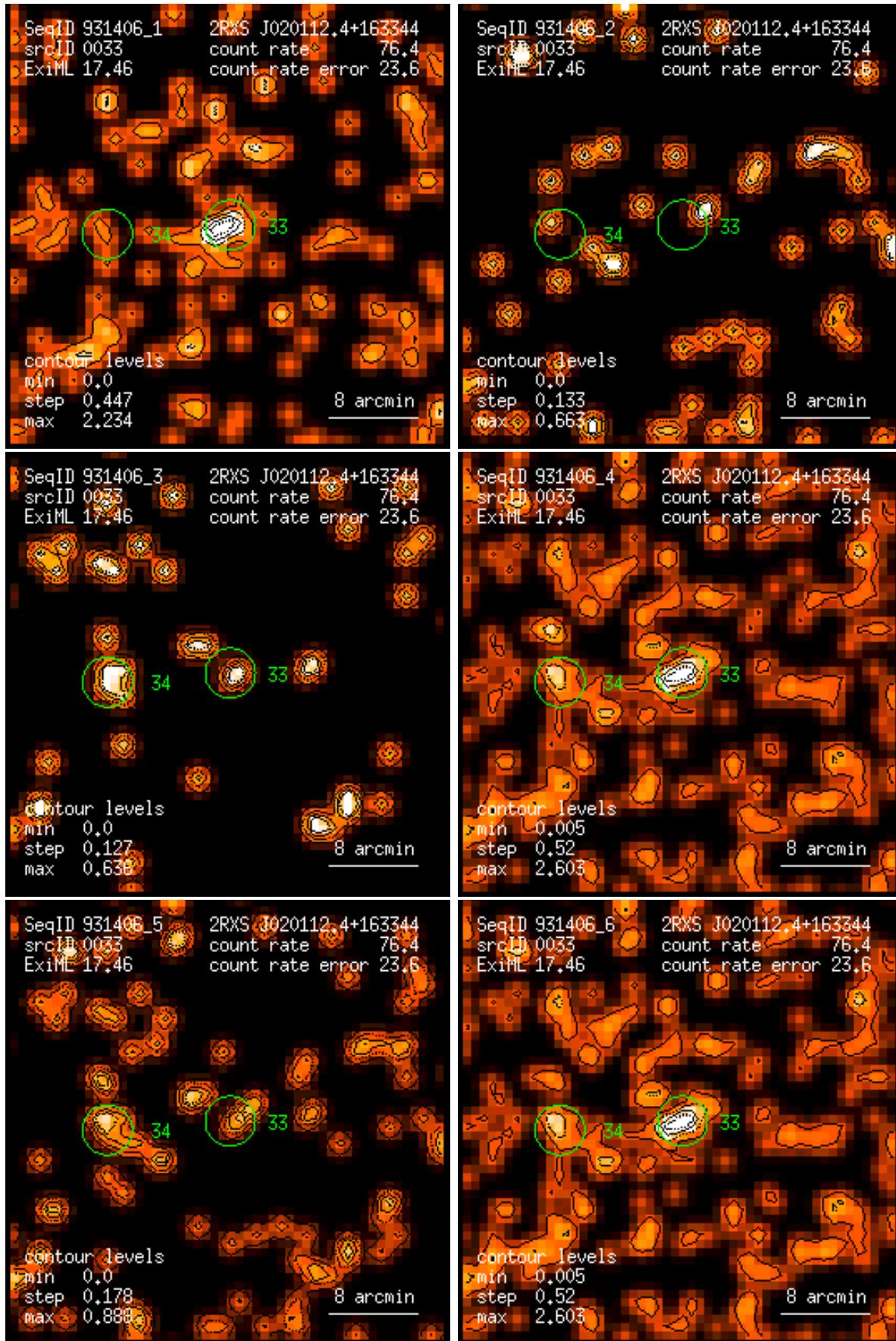
Figure 33: RASS 931406: detection 0033: band rate images, Gaussian filter: (1) PSPC channels 11 – 41, (2) 52 – 90, (3) 91 – 201, (4) 11 – 235, (5) 52 – 201, (6) 11 – 201. Broad band rates in counts/ks. Band rate contour levels in counts/ks/arcmin 2 .
