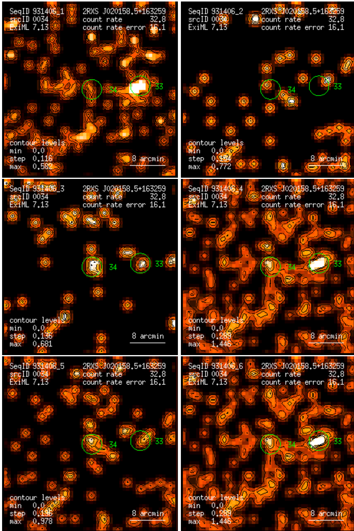
Figure 34: RASS 931406: detection 0034: band rate images, Gaussian filter: (1) PSPC channels 11 – 41, (2) 52 – 90, (3) 91 – 201, (4) 11 – 235, (5) 52 – 201, (6) 11 – 201. Broad band rates in counts/ks. Band rate contour levels in counts/ks/arcmin 2 .
