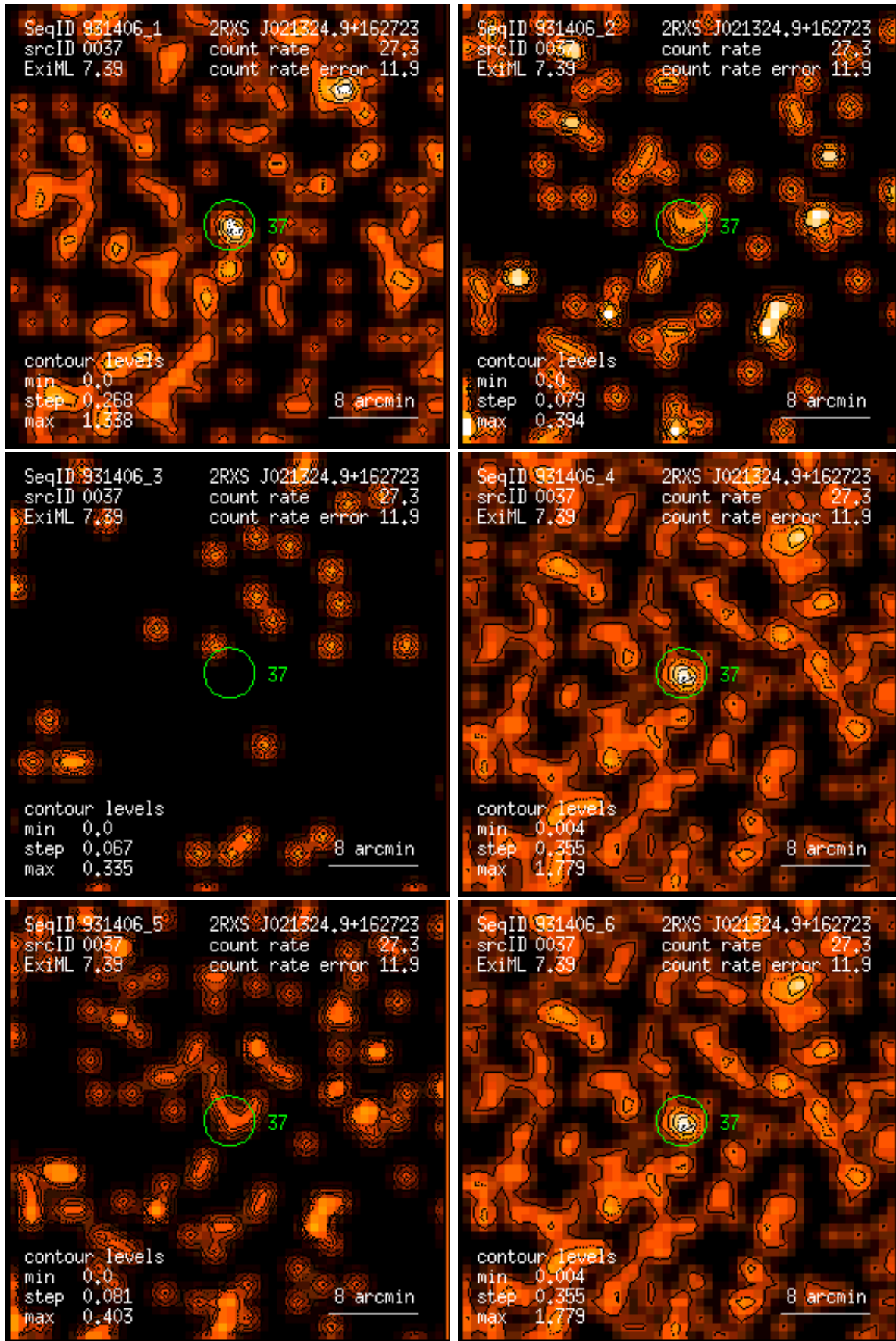
Figure 37: RASS 931406: detection 0037: band rate images, Gaussian filter: (1) PSPC channels 11 – 41, (2) 52 – 90, (3) 91 – 201, (4) 11 – 235, (5) 52 – 201, (6) 11 – 201. Broad band rates in counts/ks. Band rate contour levels in counts/ks/arcmin 2 .
