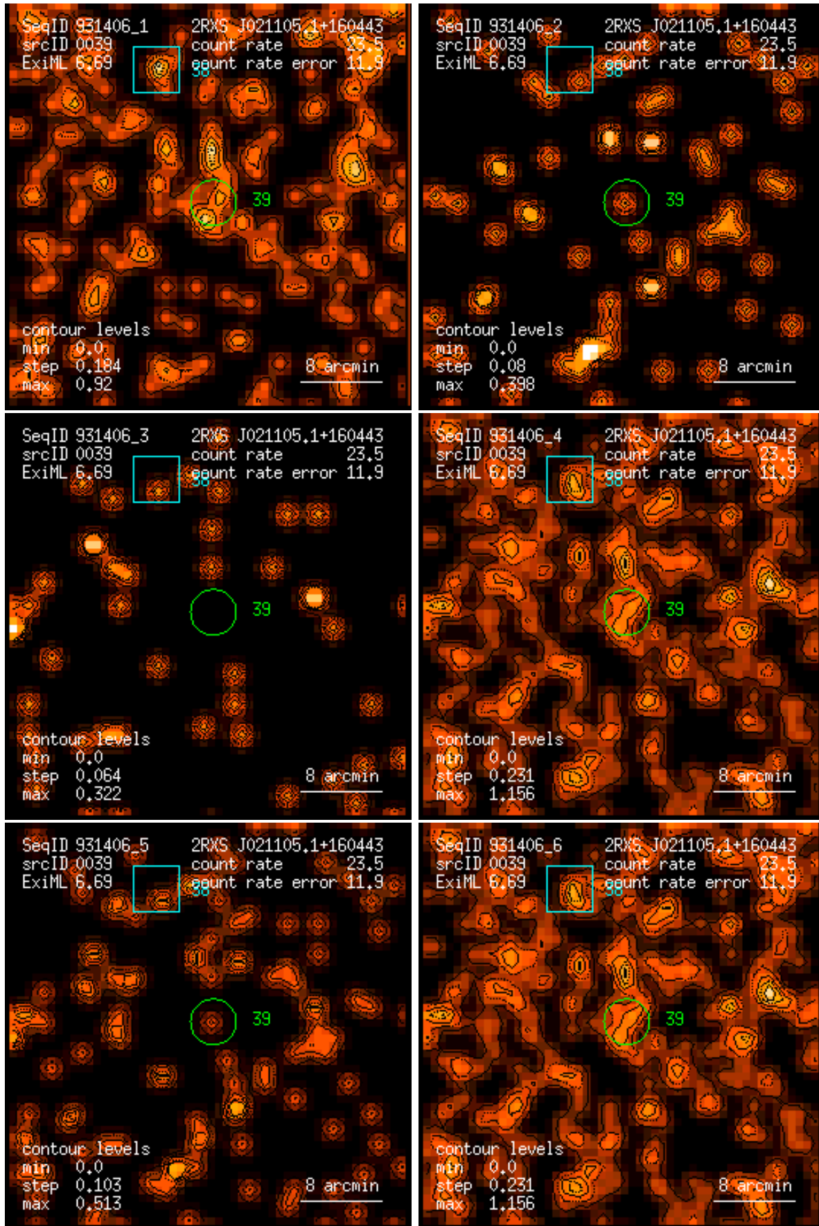
Figure 39: RASS 931406: detection 0039: band rate images, Gaussian filter: (1) PSPC channels 11 – 41, (2) 52 – 90, (3) 91 – 201, (4) 11 – 235, (5) 52 – 201, (6) 11 – 201. Broad band rates in counts/ks. Band rate contour levels in counts/ks/arcmin 2 .
