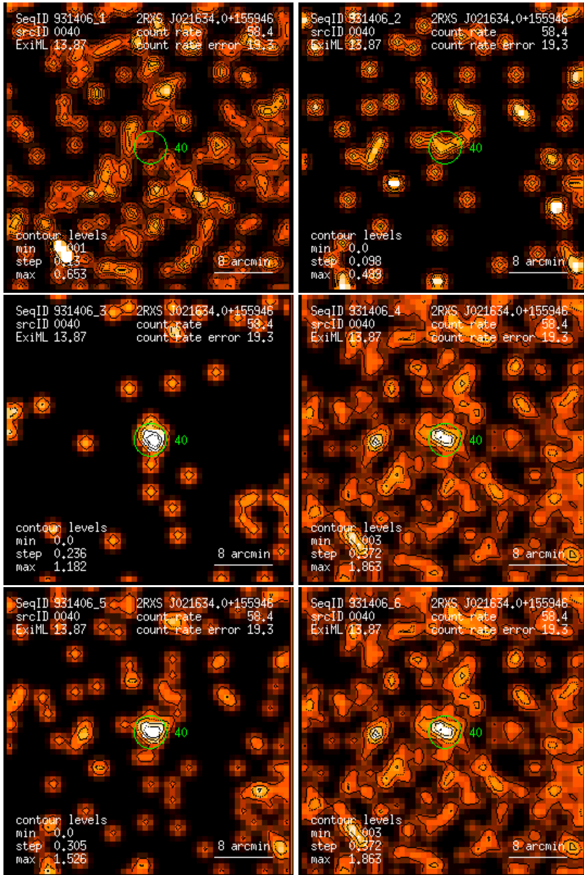
Figure 40: RASS 931406: detection 0040: band rate images, Gaussian filter: (1) PSPC channels 11 – 41, (2) 52 – 90, (3) 91 – 201, (4) 11 – 235, (5) 52 – 201, (6) 11 – 201. Broad band rates in counts/ks. Band rate contour levels in counts/ks/arcmin 2 .
