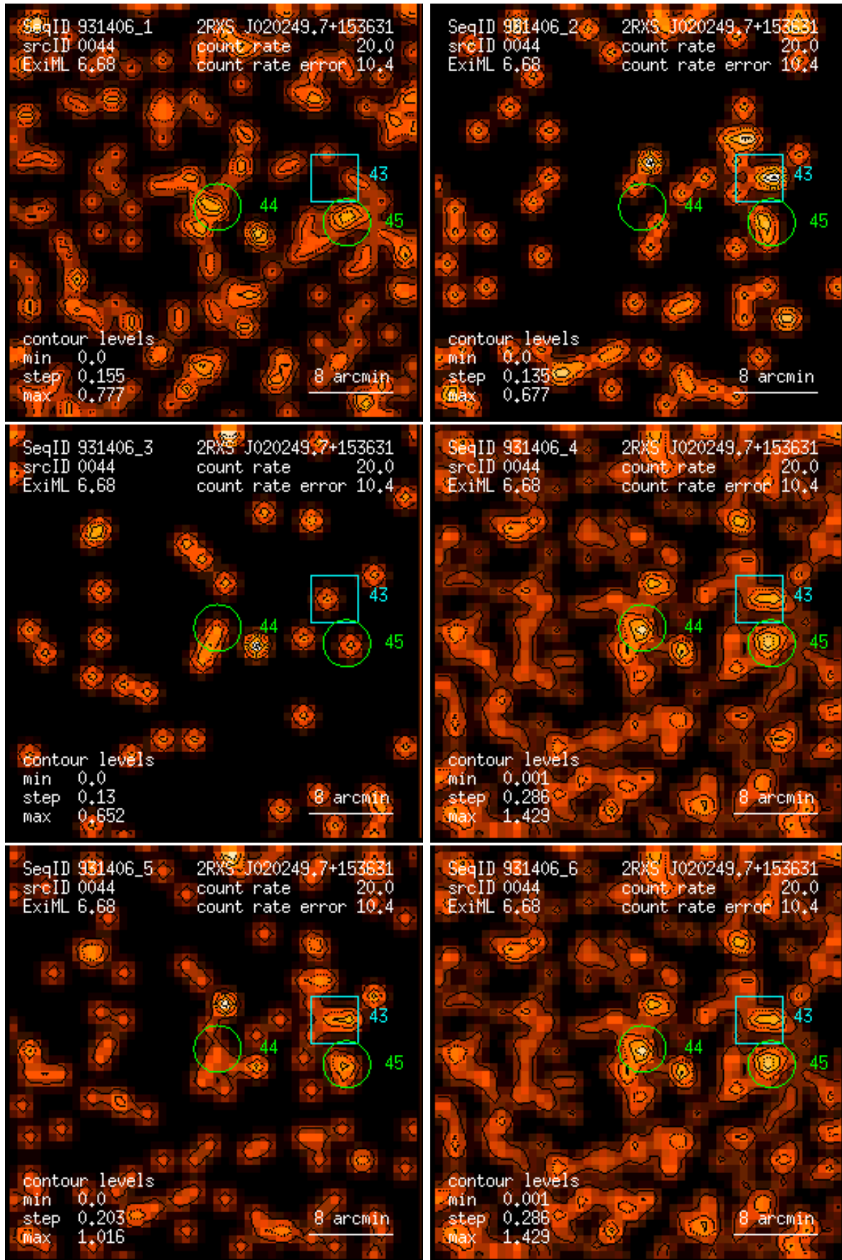
Figure 44: RASS 931406: detection 0044: band rate images, Gaussian filter: (1) PSPC channels 11 – 41, (2) 52 – 90, (3) 91 – 201, (4) 11 – 235, (5) 52 – 201, (6) 11 – 201. Broad band rates in counts/ks. Band rate contour levels in counts/ks/arcmin 2 .
