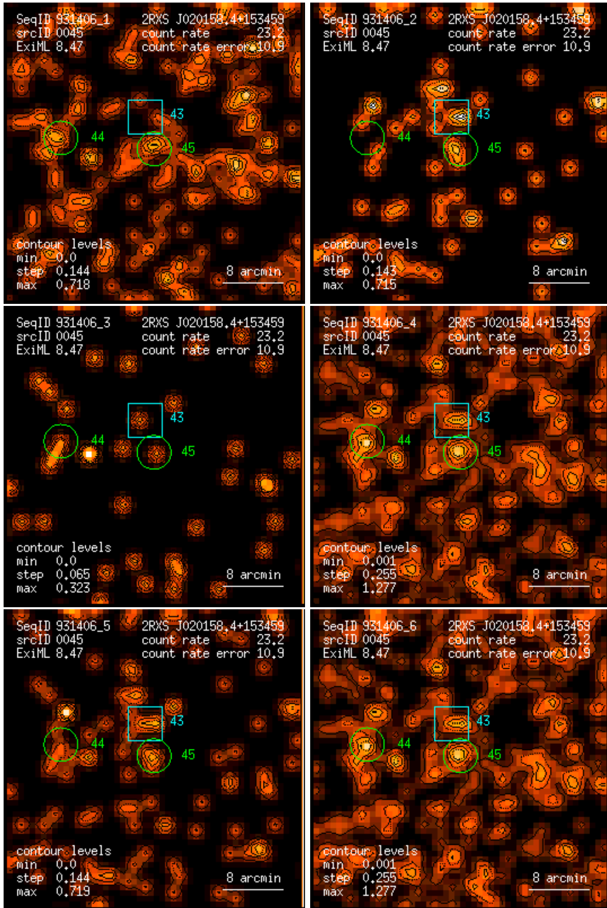
Figure 45: RASS 931406: detection 0045: band rate images, Gaussian filter: (1) PSPC channels 11 – 41, (2) 52 – 90, (3) 91 – 201, (4) 11 – 235, (5) 52 – 201, (6) 11 – 201. Broad band rates in counts/ks. Band rate contour levels in counts/ks/arcmin 2 .
