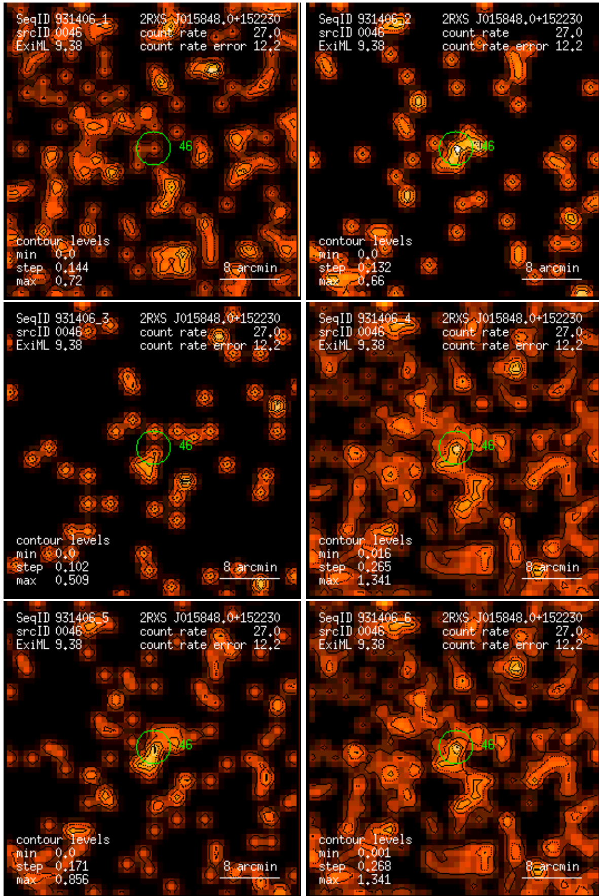
Figure 46: RASS 931406: detection 0046: band rate images, Gaussian filter: (1) PSPC channels 11 – 41, (2) 52 – 90, (3) 91 – 201, (4) 11 – 235, (5) 52 – 201, (6) 11 – 201. Broad band rates in counts/ks. Band rate contour levels in counts/ks/arcmin 2 .
