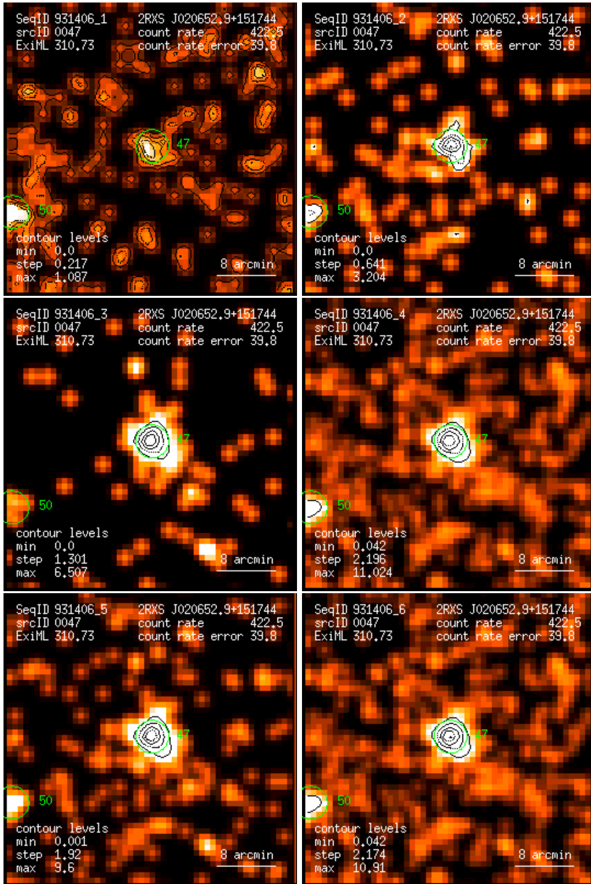
Figure 47: RASS 931406: detection 0047: band rate images, Gaussian filter: (1) PSPC channels 11 – 41, (2) 52 – 90, (3) 91 – 201, (4) 11 – 235, (5) 52 – 201, (6) 11 – 201. Broad band rates in counts/ks. Band rate contour levels in counts/ks/arcmin 2 .
